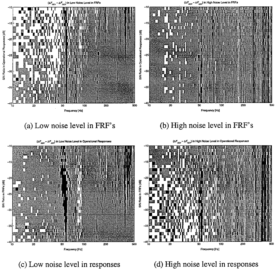
Figure 28. Comparison of average errors in forces reconstructed by OCV and GCV for various noise levels in operational responses and FRF's.
