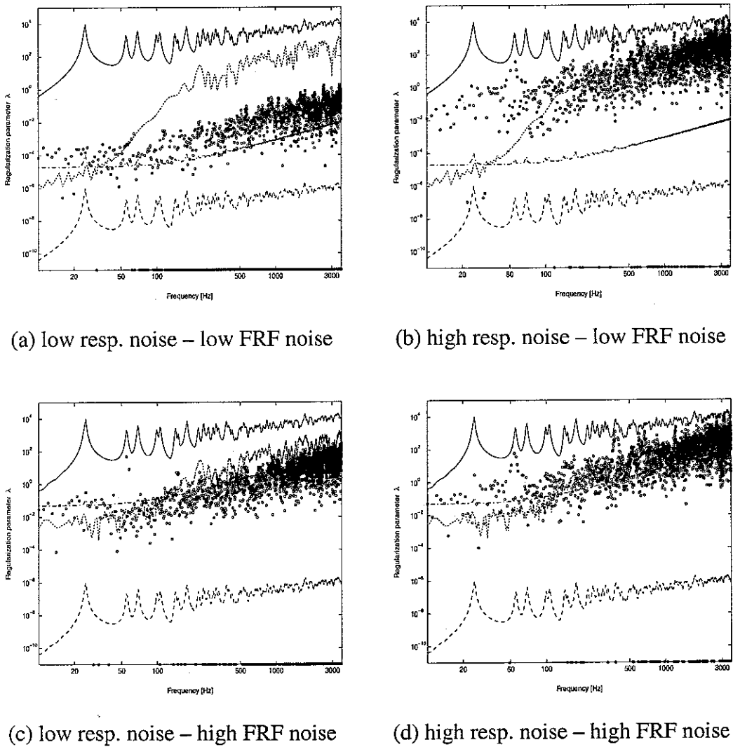
Figure 4. Regularization parameters chosen by the method of ordinary cross validation for different noise levels (○).
