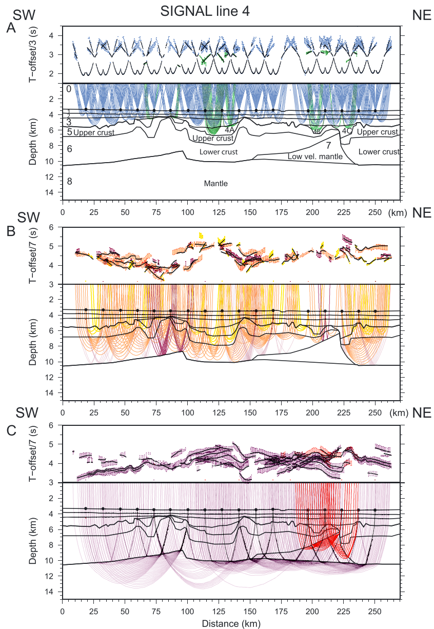
Figure 5. Ray tracing along SIGNAL Line 4. Layers are detailed in the text. (a) The blue rays and traveltime picks are direct water waves and sedimentary phases P_{s1} , P_{s2} , and P_{s3} . The green rays and traveltime picks correspond to phase P_{s4} in the deep, high-velocity basins associated with layer 4. (b) Yellow rays and traveltime picks are related to the P_{c1} phase associated with the upper crustal layer. Orange and purple rays, respectively, correspond to phases P_{c2} (lower crust) and the PmP reflection. (c) Thick red rays turn in layer 7, while purple rays represent the Pn mantle phase. Black lines superimposed on the arrival times and their uncertainties are the calculated traveltimes from the final model (see Figure 9).
