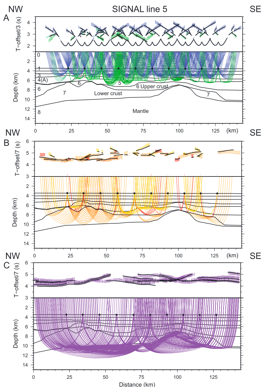
Figure 6. Ray tracing along SIGNAL Line 5. Layer numbers are detailed in the text. (a) The blue rays and traveltime picks are direct water waves and sedimentary phases P_{s1} , P_{s2} , and P_{s3} . The green rays and traveltime picks correspond to phases P_{s4} , P_{s5} , and P^* turning in layers 4 and 5 (details in section 4). (b) Yellow rays and traveltime picks are related to the P_{c1} phase associated with the upper crustal layer. Orange and red rays correspond to phases P_{c2} (lower crust) and a crustal reflection, respectively. (c) Purple rays represent the P_n mantle phase. Black lines superimposed on the arrival times and their uncertainties are the calculated traveltimes from the final model (see Figure 9).
