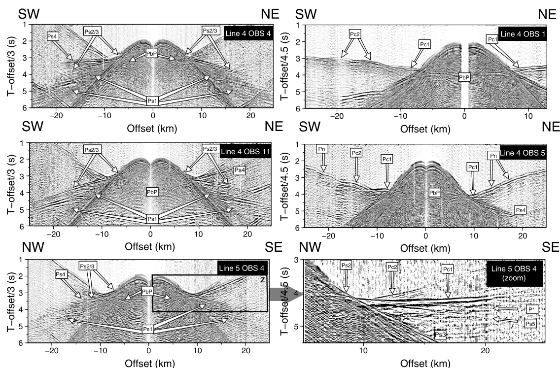
Figure 2. OBS data: sedimentary and crustal arrivals as discussed in the text. The data are band-pass filtered (6–35 Hz) and a predictive deconvolution is applied. Line 4 OBS 4 and Line 4 OBS 11 are records from the hydrophone channels, while all other records are from the vertical geophone channel. The left column uses a reduction velocity of 3 km/s to focus the display on sedimentary arrivals, while the right column uses a reduction velocity of 4.5 km/s, to focus the display on upper crustal arrivals. Phases P_{s5} and P^* on Line 5 OBS 4 have slopes indicated by the two arrows. A blow-up of the Line 4 OBS 4 reflections, including the P_xP phase is available in supplementary material Figure S1.
