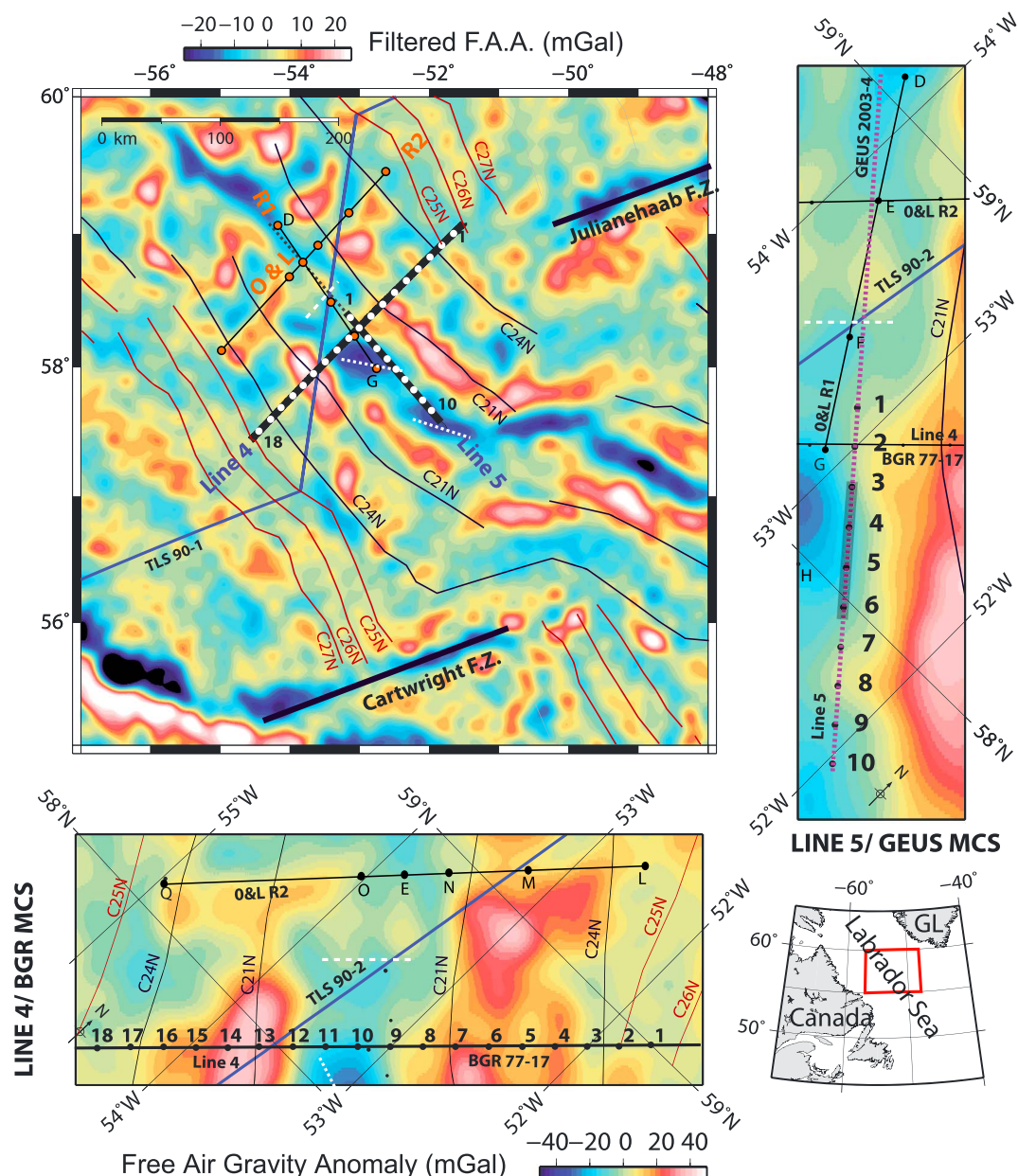
Figure 1. The extinct Labrador Sea spreading center. (top left) The background of the main map displays filtered ( <100 km) satellite free air gravity anomalies (FAA) from the DTU10 grid [Andersen et al. , 2010]. White circles represent ocean bottom seismometer (OBS) stations from the SIGNAL (Seismic Investigations off Greenland, Newfoundland and Labrador) experiment, while orange ones are OBS locations of a previous study along Lines R1 and R2 [Osler and Loudon, 1992, 1995]. (top right and bottom left) Blowups of both SIGNAL lines are displayed with an unfiltered satellite F.A.A background, and station numbers of OBS. SIGNAL Line 4 coincide with seismic Line BGR 77-17 [Hinze et al. , 1979; Chalmers and Laursen, 1995], while SIGNAL Line 5 follows the GEUS 2003-4 seismic line (dashed). The blue lines are seismic profiles TLS 90-1, TLS 90-2, and TLS 90-3 (from west to east, see Srivastava and Keen [1995]). Magnetic anomalies are from Roest and Srivastava [1989]. White dashed lines are interpreted spreading subsegments and transform fault (compare with Figure 15). Thick solid black lines represent major fracture zones (FZ). GL: Greenland.
