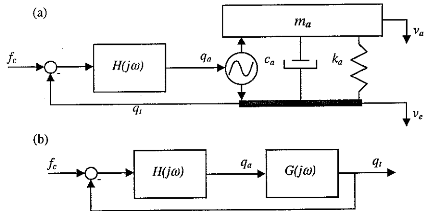
Figure 4 Schematic of an inertial actuator and implementation of the inner total transmitted force feedback control (a), and equivalent block diagram (b).
