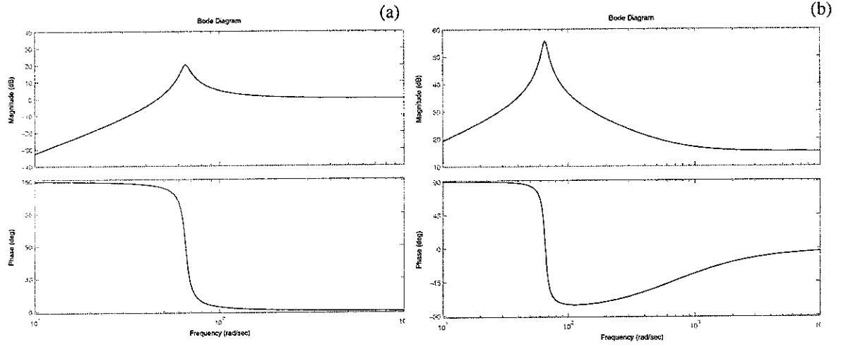
Figure 3 Magnitude and phase of the blocked frequency response of the inertial actuator (a), and magnitude and phase of the frequency response of the passive components of the inertial actuator ( Z_{open} in Equation (2)).
