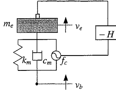
Figure 1. A simplified model of velocity feedback control
