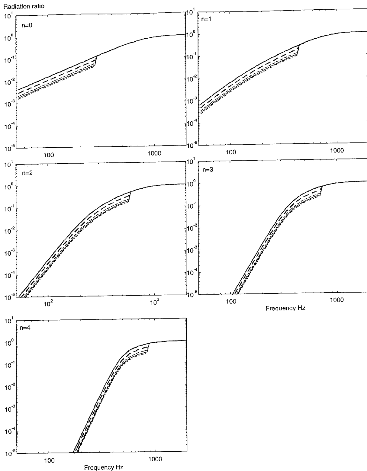
Figure 5.7 Radiation ratios predicted using simple formulae for straight webbed 0.42 m radius wheels. — normal wheel, --- double thickness tyre, ..... half thickness tyre, in grey: — full web, --- wide web.
