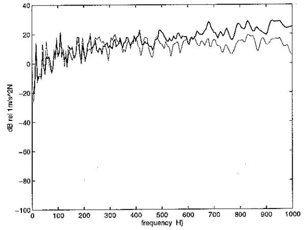
Figure 22: Estimate of the source K_{E_s} (solid line) and receiver K_{E_r} (faint) kinetic energy when the primary force F_{p3} is exciting the two panel system with three aluminium mounts with block masses and an inertial control force.
