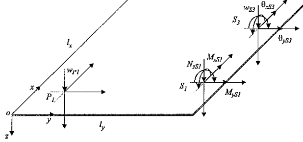
Figure A1: Notation of the displacement w at positions P_1 and S_3 , and of the rotations \theta_x and \theta_y at positions S_3 when a plate is excited in flexure by a point force N_z and point moments M_x and M_y at position S_1
