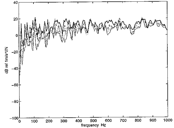
Figure 23: Estimate of the receiver K_{E_r} kinetic energy when the primary force F_{p3} is exciting the two panel system with three aluminium mounts with block masses and an inertial control force. Solid line, without control; faint line, when total power is minimised; dotted line, when forces are cancelled; dash-dotted line when velocities are cancelled.
