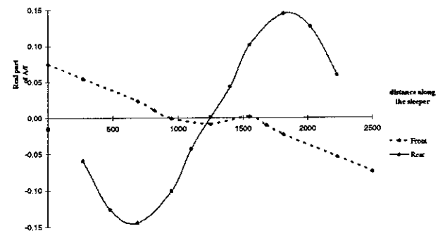
Mode shape at 382 Hz
