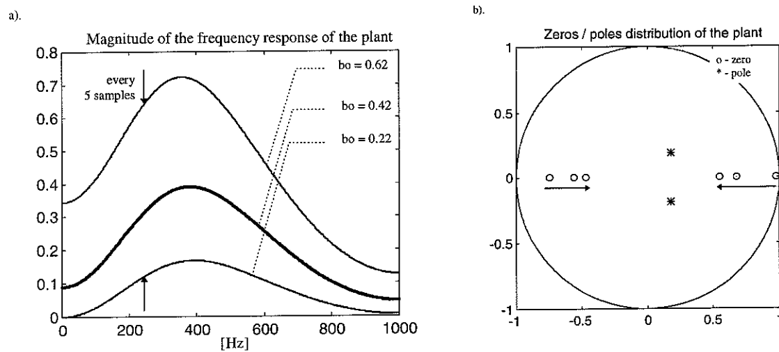
Fig. 18 The nonstationary plant:
