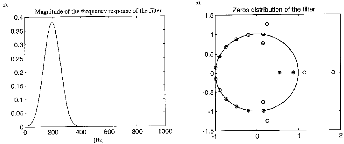
Fig. 17 The disturbance shaping filter:
