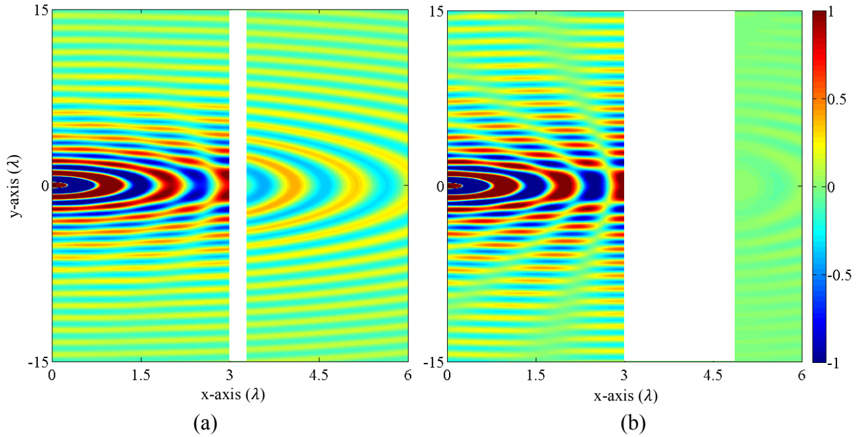
Fig. 4 – Pressure field using the equivalent source method to simulate an ‘infinite’ wall for (a) kw = 0.03 and (b) kw = 0.22 , without regularisation.
