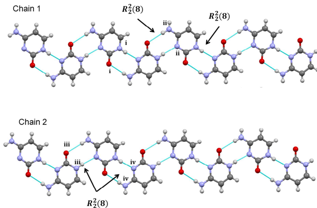
Figure 5: Chains formed by each crystallographically-independent cytosine. R_2^2(8) homosynthon is generated with symmetry equivalent counterparts of each cytosine with the following symmetry operations: i=(-x, y-0.5, -z+1.5) ; ii=(-x, y+0.5, -z+1.5) ; iii=(-x+1, y-0.5, -z+0.5) ; iv=(-x+1, y+0.5, -z-0.5) .
