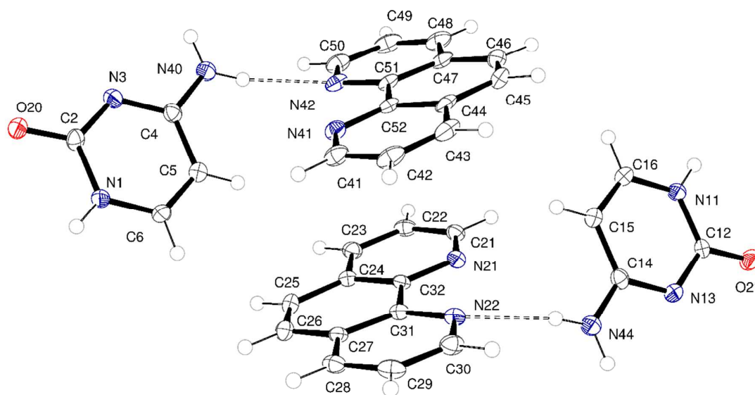
Figure 4: Asymmetric unit of cyt:phen. Atoms are drawn as 50% probability ellipsoids. Dashed lines represent N—H \cdots N hydrogen bonds
