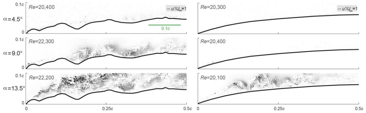
Fig. 4. Velocity vectors of the flow fluctuation field ( u' , v' ) confirm that surface roughness promotes boundary layer mixing. At \alpha = 4.5^\circ the flow over the rough surface is essentially laminar, but at higher angles there is substantial unsteady boundary layer mixing. Boundary layer mixing due to fluctuations are not apparent for the smooth airfoil at \alpha = 4.5^\circ and 9.0^\circ . At 13.5^\circ the laminar separation bubble forms a source of unsteady fluctuations, which are qualitatively of lower intensity than the ones generated by the rough surface. (Reference vector length, compared to the free stream velocity, is provided in the gray box.)
