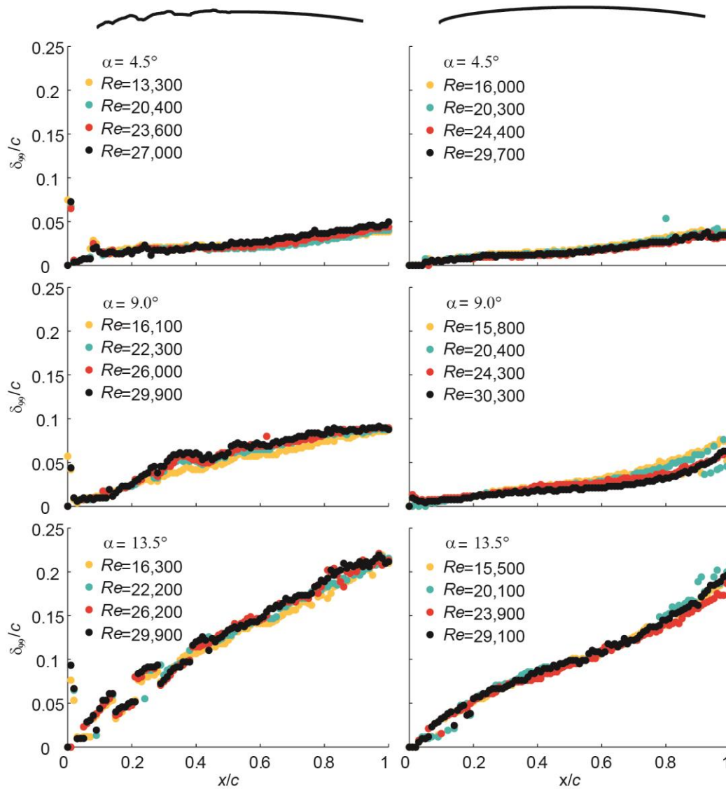
Fig. 7. Boundary layer thickness (as a proportion of chord) is similar to swift wing roughness. Boundary layer thickness, \delta_{99} , increases with relative chord position x/c and is not very sensitive to Reynolds number, instead depending primarily on \alpha and roughness. At \alpha = 4.5^\circ and 9.0^\circ , \delta_{99} is close to 0.02 (2%) chord length for the rough and smooth surface. At \alpha = 9.0^\circ , the boundary layer over the rough surface quickly increases thickness beyond x/c = 0.2 due to mixing induced by the surface roughness (Fig. 4). The surface roughness of the swift wing is thus equivalent to boundary layer thickness over the smooth airfoil (at the location of this roughness) and over the rough airfoil at \alpha = 4.5^\circ and up to x/c = 0.2 for \alpha = 9.0^\circ .
