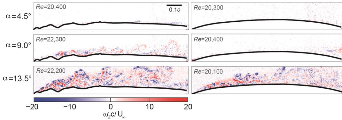
Fig. 3. Instantaneous vorticity plot based on the flow fluctuation field ( u' , v' ) shows that the flow is laminar over the rough and smooth surface at low \alpha at cruise Re of swifts. Comparison of rough and smooth surface effects for \alpha = 9.0^\circ suggest that the surface roughness indeed forms a source of vorticity fluctuation in the shear layer. At \alpha = 13.5^\circ both the smooth and rough surfaces generate extensive vorticity fluctuations in the boundary layer, but qualitatively the vorticity fluctuations appear to be more broadly distributed for the rough surface.
