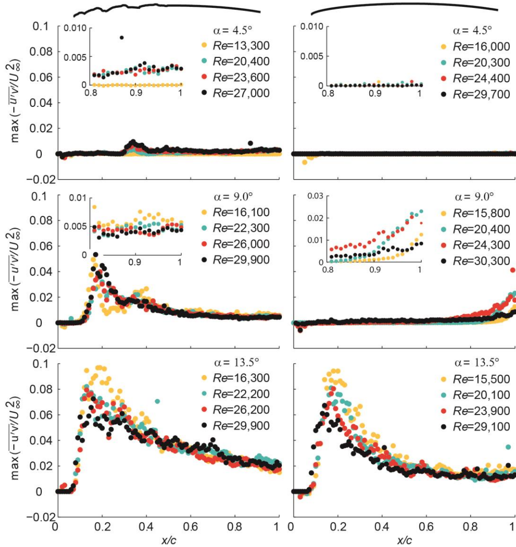
Fig. 9. Swift feather roughness generates significant Reynolds shear stresses of order 0.01 and up, a signature of transitional turbulent flow. At \alpha = 9.0^\circ and 13.5^\circ the roughness generates vortices (Fig. 4) that strongly enhance mixing and thus generate Reynolds shear stress. The smooth and rough surface only generate similar Reynolds shear stress at \alpha = 13.5^\circ , when the shear layer separates on the smooth airfoil and becomes turbulent above a laminar separation bubble (Fig. 2, 3, 4, 7). The chordwise Reynolds shear stress production is weakly dependent on Reynolds number, except for the Rough surface at \alpha = 4.5^\circ where it locally jumps from zero to non-zero when Re increases from 13,300 to 20,400.
