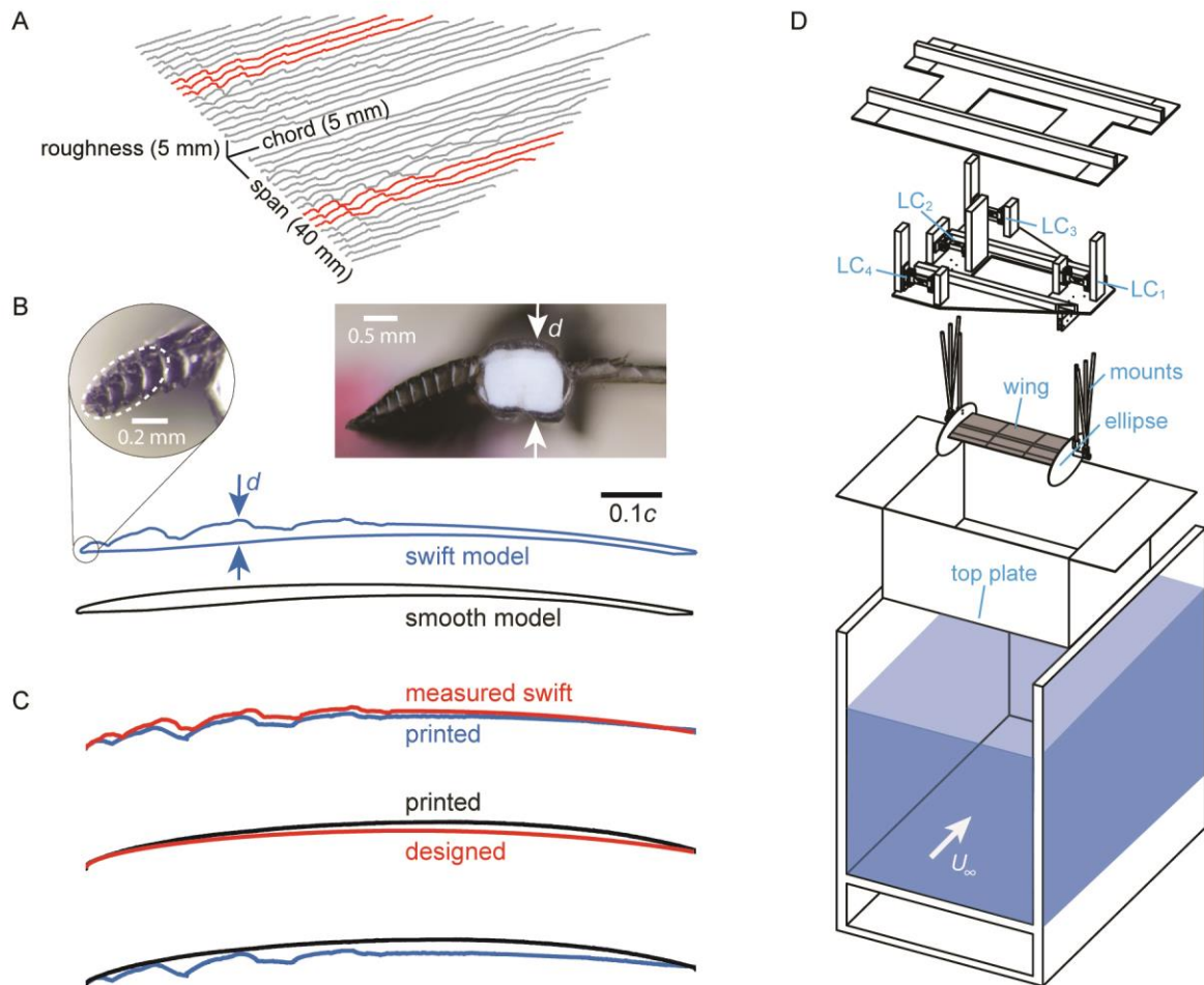
Fig. 1. Design of the 3D printed swift-like airfoil with a corrugated versus smooth surface. (A) Measured roughness profiles of a swift wing at 10 mm intervals show that the maximal roughness height occurs on the hand wing (three scan lines indicated in red, left and right). The x (chord), y (roughness), and z-axis (span) are scale bars of which the length is indicated between parentheses. (B) Rough vs. smooth swift-like airfoil, the smooth airfoil is based on the average upper surface camber of the rough airfoil. The leading edge design of both airfoils is based on a microscopy image of the cross-section of the leading-edge primary-feather of the swift hand wing. Airfoil thickness is based on primary feather rachis diameter ( d ). (C) Average upper surface profile of the swift hand wing (measured, red versus 3D printed, blue) and smoothed profile (designed, red versus 3D printed, black). Measured differences between CAD models and printed wings are due to the 3D printing process. The tiny protrusions at the leading and trailing edge are data averaging artefacts and do not represent the surface. (D) Exploded view of the PIV and force measurement setup in a water tunnel with a 0.6 \times 0.6 \times 5.0 m test section. A top plate on the water surface suppresses the influence of surface waves, ellipse-shaped end plates reduce 3D effects, and load cells (LC) 1–4 provide force data.
