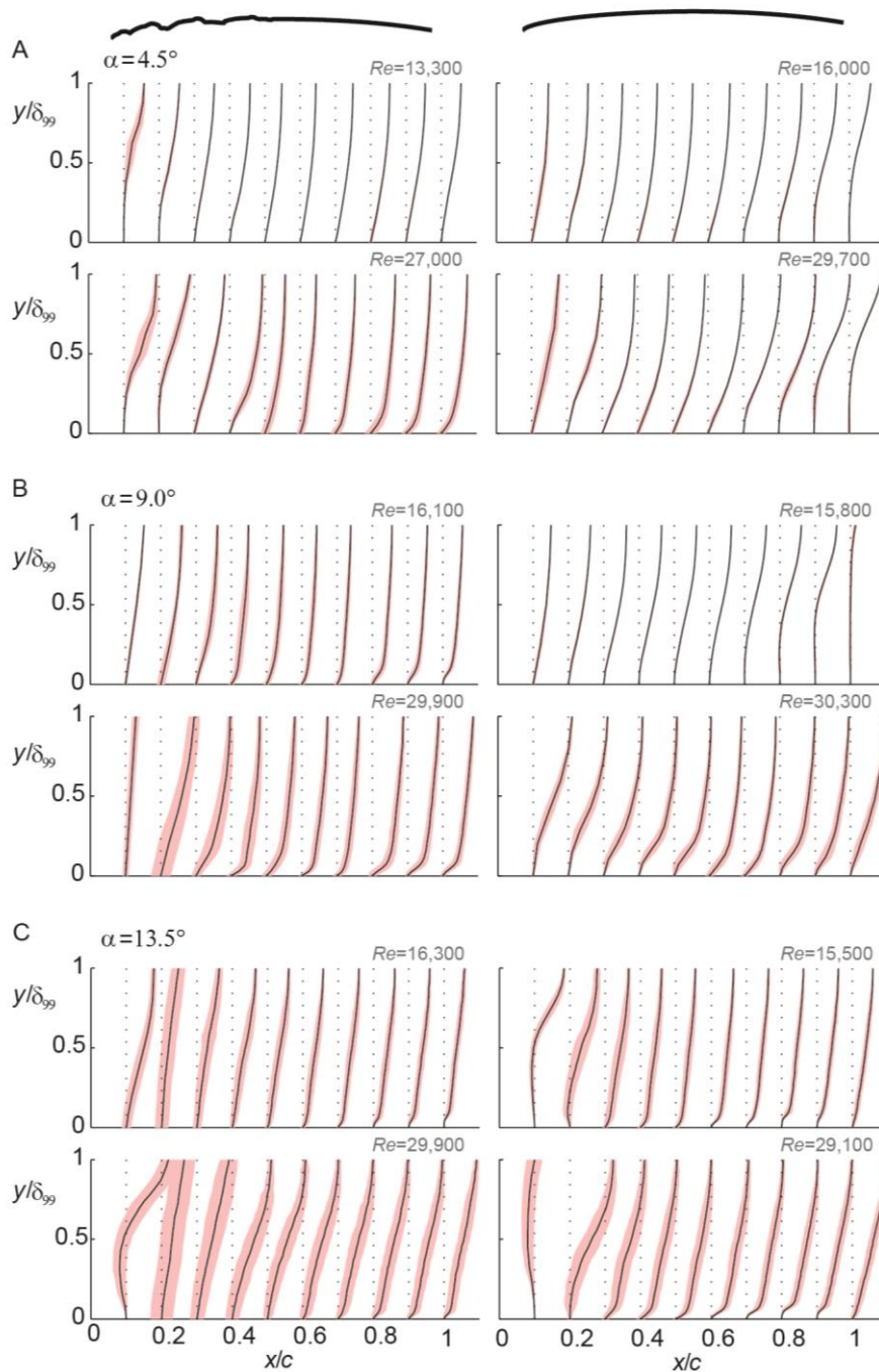
Fig. 6. Boundary layer separation is reduced by roughness, high Reynolds number, and high angle-of-attack. Boundary layer thickness, \delta_{99} , is defined based on when the velocity reaches 99% of the free stream value. Solid lines indicate the average velocity profile for different chord positions x/c , whereas the colored area indicates boundary layer profile standard deviation. An inflected boundary layer profile indicates flow separation, which can be reduced by flow fluctuations that mix the boundary layer, indicated by large standard deviation. (A, B, C) Boundary layer profiles for three different angles-of-attack, \alpha = 4.5^\circ , 9.0^\circ , and 13.5^\circ , at the minimum vs. maximum Reynolds number tested for the rough and smooth surface. The non-zero velocity standard deviation at the surface of the pronounced corrugation is due to PIV limitations.
