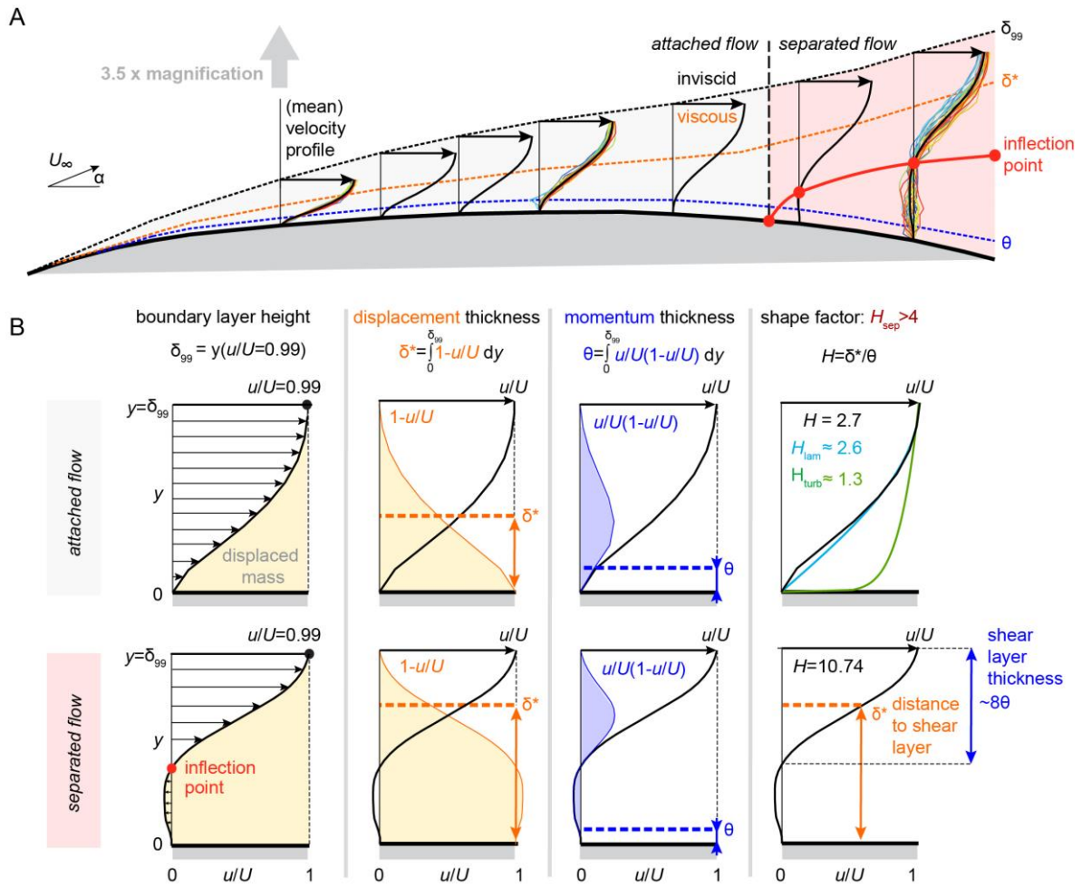
Fig. 5. Explanatory figure showing idealized boundary layer flow development over the smooth wing to help introduce the boundary layer parameters used in figure 6-8. This figure and its explanations are adapted from (White, 1991) and (Drela, 2014). (A) Illustration of boundary layer flow over the smooth wing using average (black) and instantaneous (rainbow) flow profiles measured at \alpha = 9.0^\circ and Re = 20,400 . The development of the boundary layer ( U_\infty , free stream velocity) from the leading to trailing edge is characterized by the boundary layer thickness ( \delta_{99} ; black dashed line), the displacement thickness ( \delta^* ; orange dashed line), the momentum thickness ( \theta ; blue dashed line), and the inflection points (red dots connected by red line). For clarity we magnified the vertical axis in the boundary layer with a factor 3.5. (B) Graphical illustration of the integral boundary layer parameters that characterize boundary layer development, local laminar versus turbulent attached flow, and flow separation (Drela, 2014). Boundary layer height, \delta_{99} , is the vertical position at which the flow reaches 99% of the free-stream velocity ( y , wall normal; u , local tangential velocity; U , tangential velocity at edge of boundary layer). Displacement thickness, \delta^* , is a measure for how far the main flow is pushed away from the surface. The momentum thickness, \theta , is a measure for how far the momentum of the main flow is pushed away from surface. Shape factor, H , is the ratio of displacement and momentum thickness, and characterizes the shape of the velocity profile for attached laminar ( H_{turb} \approx 1.3 ) and turbulent ( H_{lam} \approx 2.6 ) flow. For separated flows the corresponding shape factor is H_{sep} > 4 and \delta^* is a measure for how far the shear layer is separated from the wall, while the thickness of the separated shear layer can be estimated as 8\theta (Drela, 2014). For brevity we write U in panel B instead of the equivalent U_\infty .
