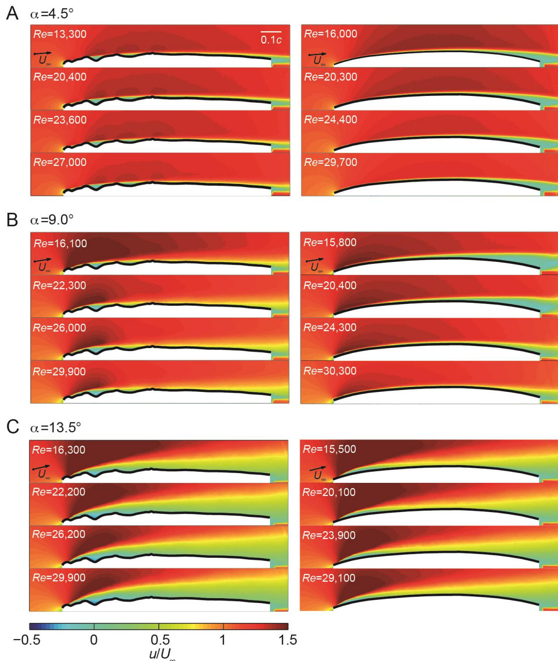
Fig. 2. Averaged flow fields for a swift-like airfoil with feather roughness (left) versus a smooth surface (right) as a function of Re and \alpha . (A) At \alpha = 4.5^\circ the flow over the rough airfoil ( left ) separates and recirculates in the valleys between the rachis bumps, but beyond the biggest bumps it remains attached till the trailing edge. The flow over the smooth airfoil ( right ) remains attached until about 70% chord length, after which the flow separates beyond the trailing edge. (B) At \alpha = 9.0^\circ the flow over the rough airfoil ( left ) also remains attached until the trailing edge. At low Re , the flow over the smooth airfoil ( right ) separates beyond about 50% chord length, but at high Re the flow separation is much reduced. (C) At \alpha = 13.5^\circ the flow over both the rough and smooth wing remain attached
