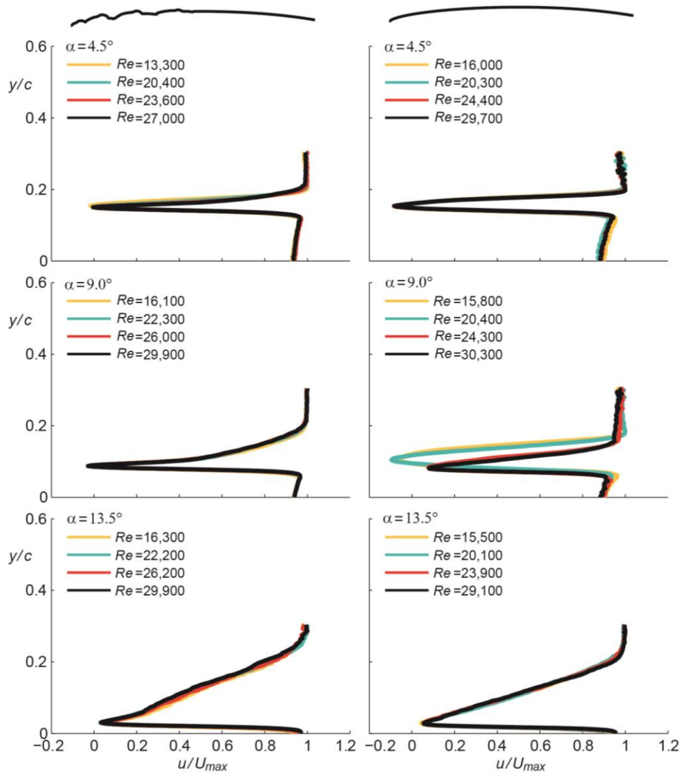
Fig. 10. Wake velocity deficit profiles at x/c = 1.05 (5% behind the trailing edge), show the wake generated by the rough surface is similar across Re . The boundary layer over the upper surface dictates the development of the upper part of the wake profile, which depends on \alpha . The wake profile behind the smooth airfoil is Re sensitive at \alpha = 9.0^\circ due to flow separation over the smooth surface (Fig. 5).
