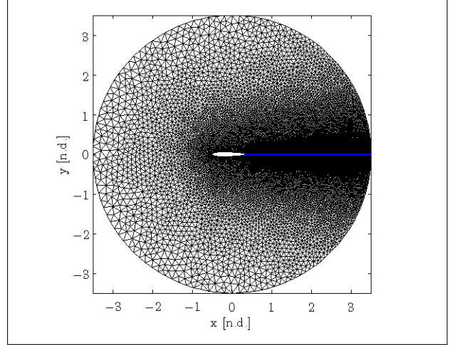
Figure 2. Aerodynamic mesh. Domain extent associated to \alpha = 6^\circ .
