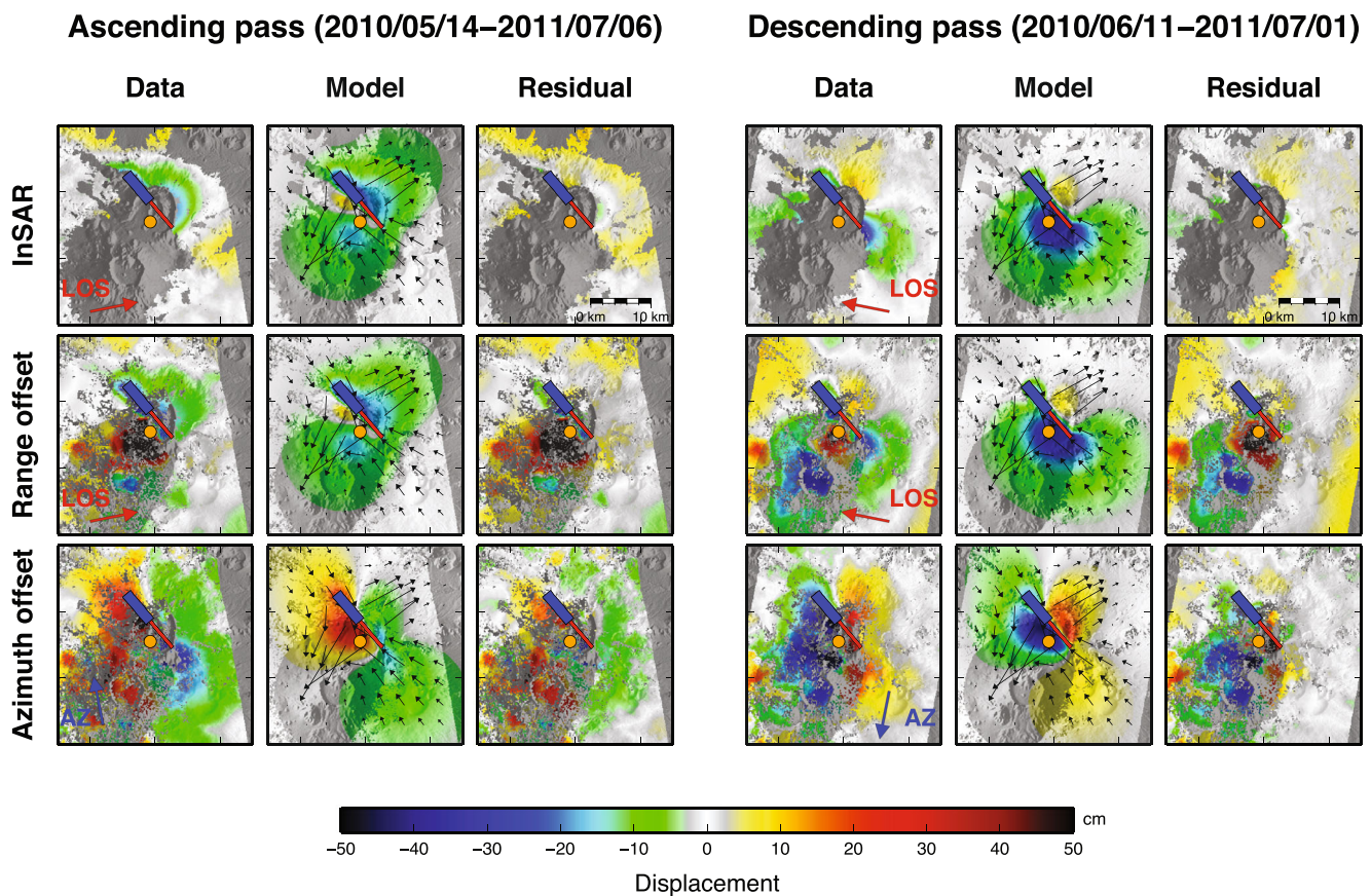
Fig. 3 Comparison of observed ( Data ), predicted ( Model ) and residual ( Residual ) deformation for the various components of ground motion deduced from ascending ( left panel ) and descending ( right panel ) SAR data. The top row corresponds to InSAR, the middle row to range offsets and the lower row to azimuth offsets. The thick-coloured arrows show the direction of sensed ground displacement: red for line-of-sight (LOS) and blue for along-track (AZ). InSAR and range offsets are sensitive to motion only in the LOS direction. The LOS vector makes an angle of 29^\circ with the vertical for the ascending pass ( 34^\circ for the descending pass). For clarity, only the horizontal component of the LOS vector is shown by the red arrow . In contrast, azimuth offsets only provide information on the horizontal component of ground motion in the direction of the satellite
