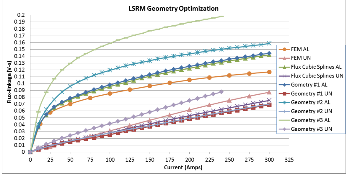
Fig. 8. Flux linkages for the aligned and unaligned positions using flux cubic-splines and FEA.
