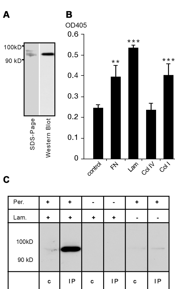
Fig. 6. Interaction of periostin with ECM molecules. (A) Periostin comprising a C-terminal His-tag and an additional c-Myc epitope was expressed in HEK-293 cells and purified by using \text{Ni}^{2+} affinity chromatography. Coomassie-stained SDS-PAGE and immunoblotting using a Myc-specific antibody revealed a protein with a molecular mass in the expected range of slightly above 90 kDa. (B) Interaction of periostin with ECM molecules was analysed by using a solid-phase assay. 100 \mu\text{g}/\text{ml} of the ECM molecules were coated onto 96-well plates and incubated with 50 \mu\text{g}/\text{ml} recombinant periostin in the presence of \text{Ca}^{2+} in the binding buffer. Interaction of periostin was detected using an anti-c-Myc HRP conjugate and visualized using ABTS as a substrate. Note that the interaction was \text{Ca}^{2+} -dependent as binding in the absence of \text{Ca}^{2+} was below the control level and did not vary between the different ECM molecules. Significance is indicated as ** P < 0.01 , *** P < 0.001 . FN, fibronectin; Lam, laminin; Col, collagen (isoforms IV and I, respectively). (C) Co-immunoprecipitation of laminin (Lam.) and periostin (Per.) was performed in mock (–) or periostin (+) transfected HEK-293 cells. Laminin (+) was added to the supernatant and complexes were precipitated using a laminin-specific antibody. The interaction was assessed by immunoblotting and detection of precipitated periostin with a Myc-specific antibody. The control lanes (c) represent the input before immunoprecipitation, whereas the ‘IP’ lanes show the results after immunoprecipitation.
