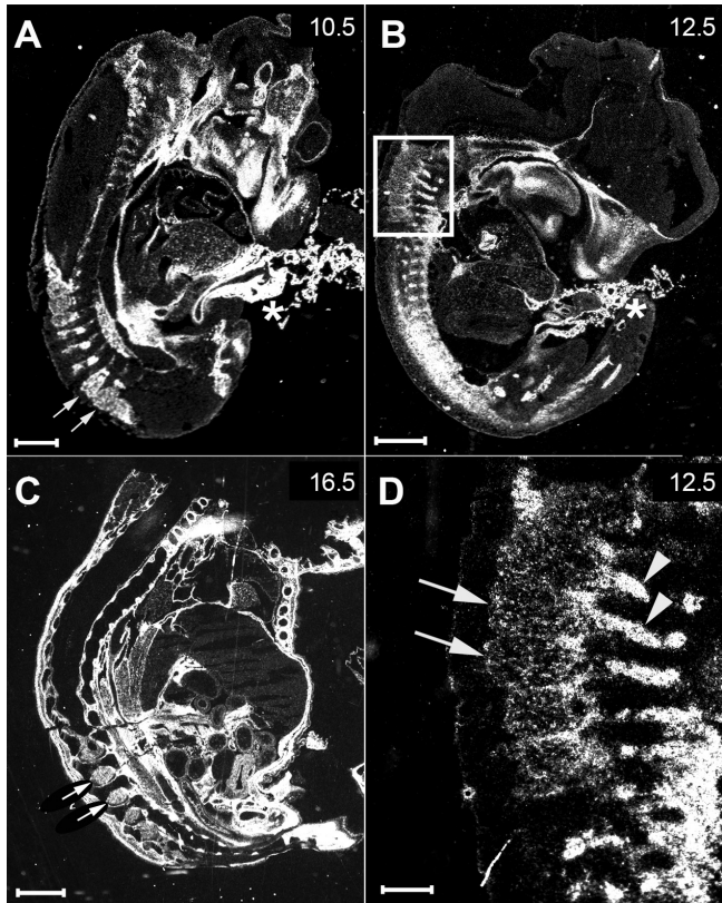
Fig. 2. Expression analysis of periostin in DRG. (A–D) Periostin expression during development was followed by using in situ hybridisation with a ^{35}\text{S} -labelled periostin-specific probe on sagittal sections of wild-type embryos at different stages. Expression in several connective tissues, the periosteum and the valves of the heart has been previously described. Also note the strong expression in the umbilical cord, highlighted with an asterisk (A,B).
