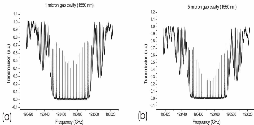
Fig. 3. (a) and (b) show the spectral responses of two gap cavities made using FBG mirrors. Typically cavity lengths are of the order of \sim cm while the air gap is <5\mu\text{m} .
