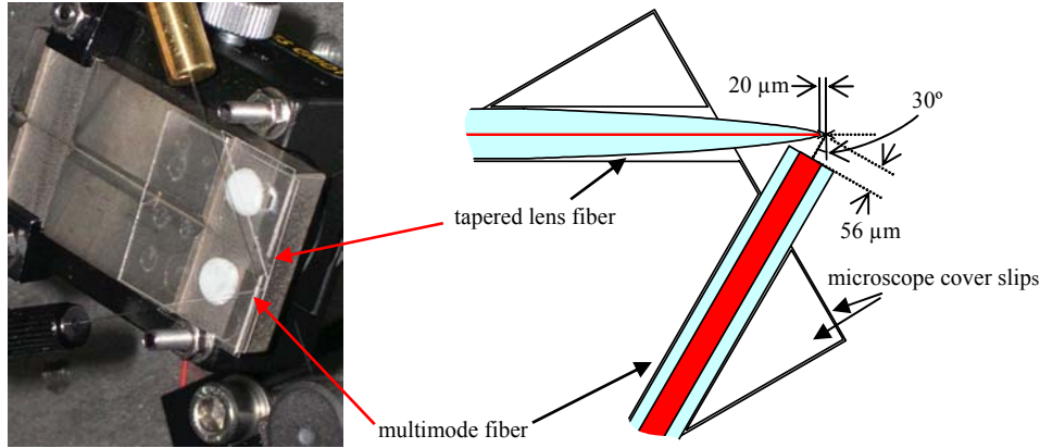
Fig.1. On the left is a photograph of the prototype atom detector described in the text and on the right is a schematic diagram of this set up.
