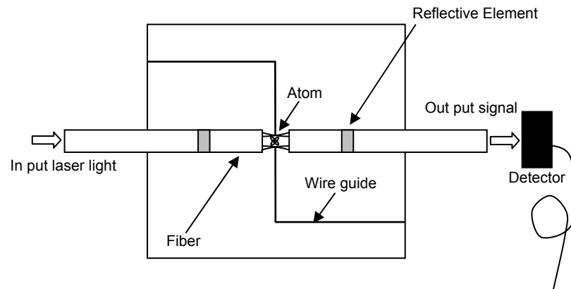
Fig. 2. A schematic diagram of a possible arrangement for on-chip atom detection.
