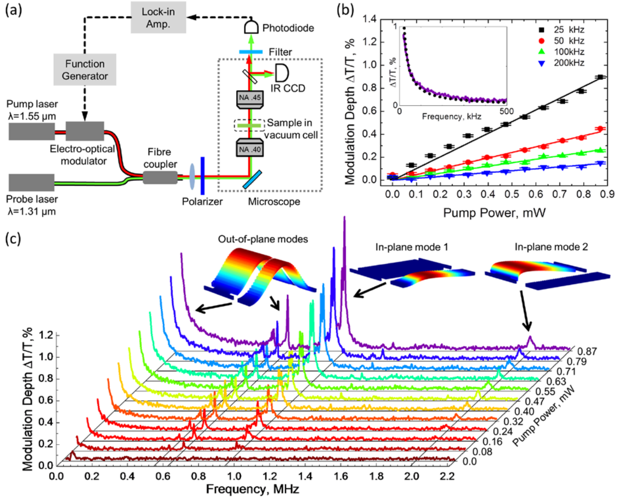
Figure 3. Modulating light with light using optically reconfigurable metamaterial. (a) Schematic of the pump-probe experimental setup. (b) Probe transmission modulation depth at \lambda = 1310 \text{ nm} as a function of pump power for several pump modulation frequencies with linear fits (solid lines). The inset shows a hyperbolic fit \sim 1/f (black dotted line) of the thermal modulation tail for a pump power of 0.9 mW. (c) Modulation depth as a function of pump laser power and modulation frequency. Corresponding mechanical modes of the metamaterial nanostructure are shown near resonant peaks. The pump modulation depth is close to 100% in all cases.
