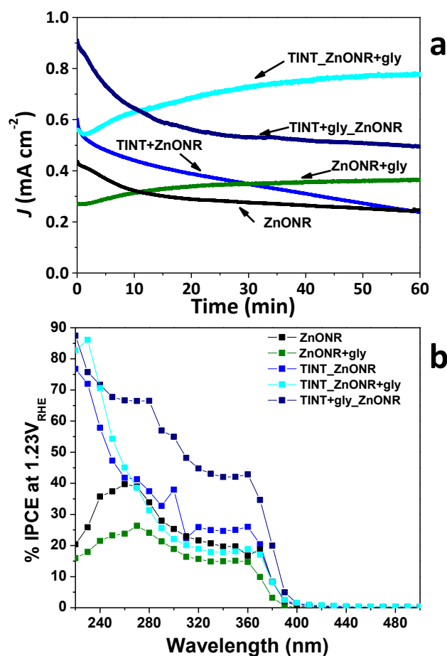
Figure 5. (a) Chronoamperometry plots ( J vs time) performed at 1.23 V_{RHE} . (b) IPCE performed at 1.23 V_{RHE} for all electrodes. Electrolyte: 0.01 mol L -1 Na 2 SO 4 .
