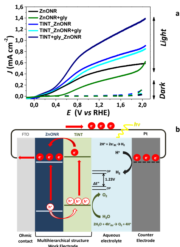
Figure 4. (a) Photocurrent ( J ) vs. voltage ( V_{\text{RHE}} ) curves without and with sunlight irradiation, measured using a scan rate of 50 \text{ mV s}^{-1} . Electrolyte: 0.01 \text{ mol L}^{-1} \text{ Na}_2\text{SO}_4 ; (b) Schematic representation of photoelectrocatalytic water splitting using the TiNT/ZnONR-based multihierarchical electrodes.
