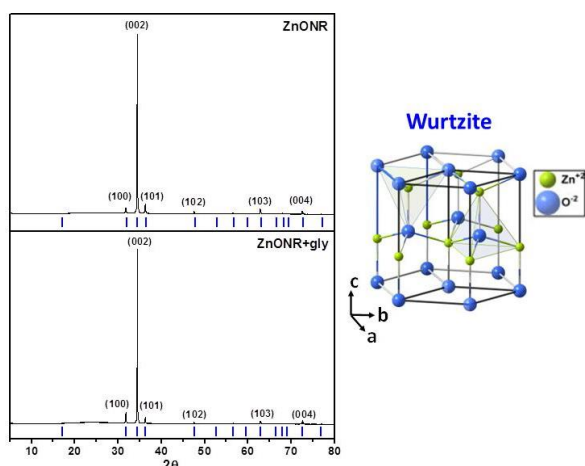
Figure 2. XRD Patterns of ZnONR and ZnONR+gly films and the crystalline structure of wurtzite.
