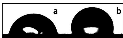
Figure 3. Contact angle images of \text{Na}_2\text{SO}_4 0.01 \text{ mol L}^{-1} aqueous solution droplet on the surface of (a) ZnONR and (b) ZnONR+gly films.
