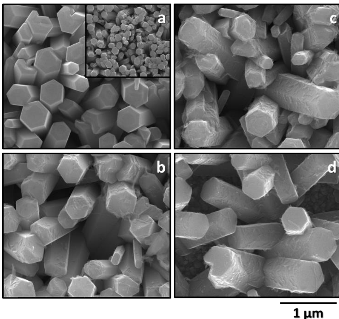
Figure 1. SEM images of (a) ZnONR, (b) TiNT→ZnONR, (c) TiNT+gly→ZnONR, and (d) TiNT→ZnONR+gly films.
