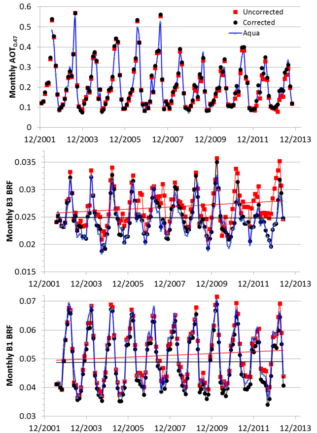
Figure 8. Effect of polarization correction on clear-sky monthly average MAIAC AOT 0.47 (top) and surface BRF in bands B3 (middle) and B1 (bottom). Different colors refer to C6 L1B MODIS Terra uncorrected (red), corrected (black) and MODIS Aqua (blue) data.
