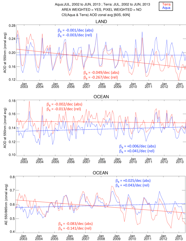
Figure 1. Time series of C5 “dark-target” monthly global mean AOD at 0.55 μm over land (top) and ocean (middle) and AE (using 0.86 and 0.55 μm) over ocean (bottom), for Terra (red) and Aqua (blue) during July 2002–June 2013. The shown linear trend slopes are given in units of AOD or AE per decade ( \beta_B ) and percentage of change per decade ( \beta_R ). Data are obtained from the monthly Level 3 product.
