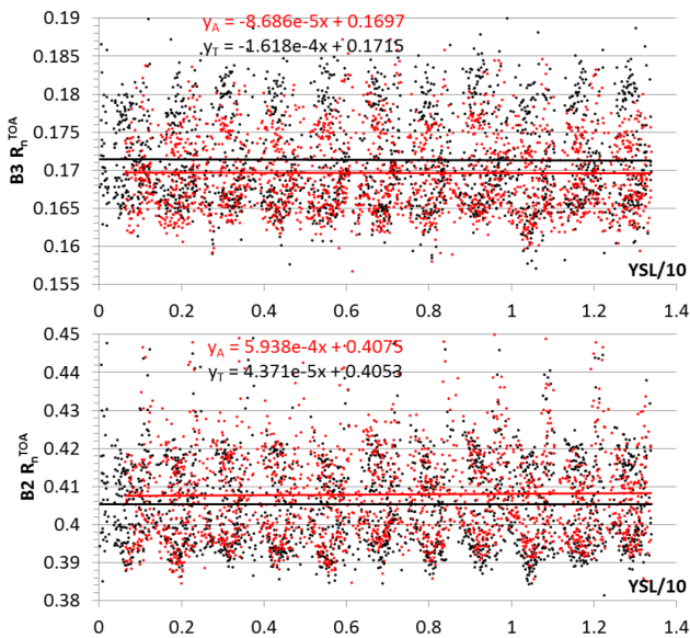
Figure 11. Clear-sky daily reflectance R_n^{TOA} over the Libya 4 site for MODIS Terra and Aqua bands B2 and B3 after detrending.
