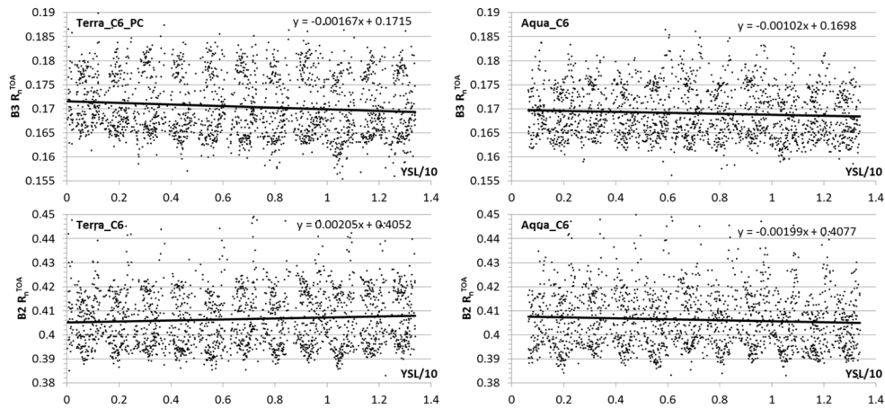
Figure 10. Derivation of detrending coefficients over the Libya 4 site for MODIS Terra and Aqua bands B2 and B3. The vertical axis shows clear-sky daily reflectance R_n^{TOA} computed for the normalized geometry, and the horizontal axis shows years since launch (YSL)/10.
