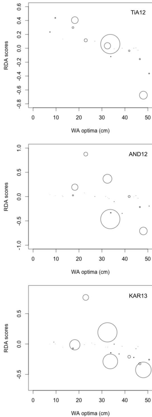
Figure 4. Abundance-weighted correlation between weighted-average optima for taxa observed in each core and RDA species scores of an ordination constrained by the WA reconstruction. TiA12: p = 0.022 ( r^2 = 0.89 ); AND12: p = 0.426 ( r^2 = 0.64 ); KAR13: p = 0.207 . RDA: redundancy analyses.
