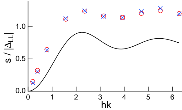
Fig. 3. Shift of the resonance s , scaled to the absolute value of the LL shift |\Delta_{LL}| , as a function of the sample thickness h , for two densities \rho = 0.01 k^3 (circles) and \rho = 0.005 k^3 (crosses). Also shown is the prediction (2), shifted up by |\Delta_{LL}| for easier comparison (solid line). The largest optical thickness in the raw data is D \simeq 1 , so for all parameter values in this figure the sample is still fairly transparent. The truncation errors in the data points are at most on the order of one per cent.
