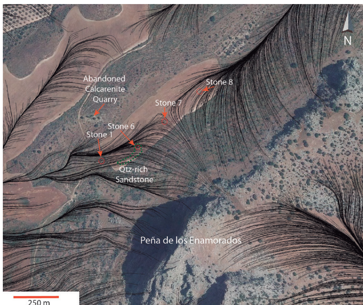
Fig. 15. Ortophotography of Piedras Blancas I and DEM-calculated accumulated flow lines of potential trajectories of stone blocks from the northern cliff of La Peña de los Enamorados by gravitational fall. Design: José Antonio Lozano Rodríguez, Luis Alfonso Pérez Valera and Fernando Pérez Valera.
