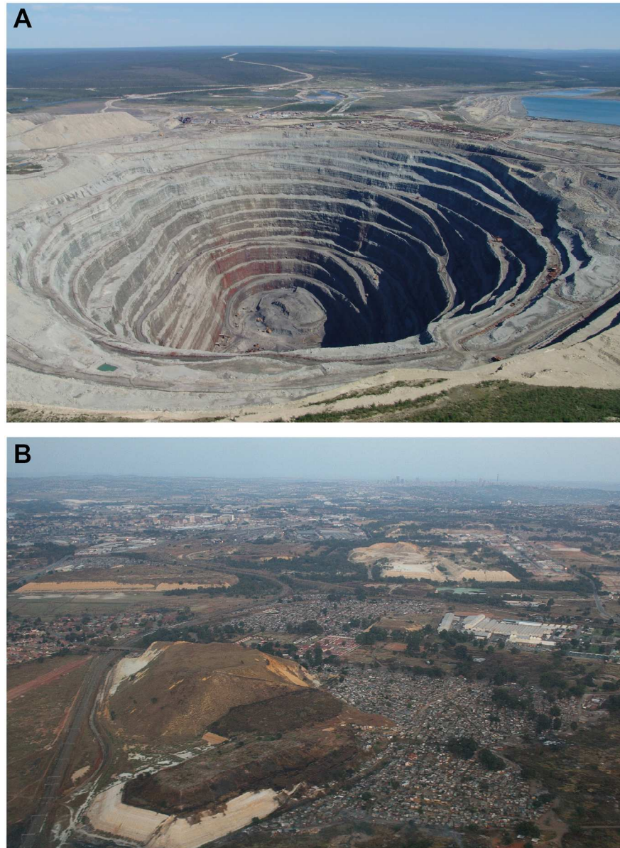
Figure 7. Oblique aerial views of mining-related landforms: A) the Udachnaya pipe, an opencast diamond mine in the Daldyn-Alakit kimberlite field in Sakha Republic, Russia. At more than 600 m deep, it is the third deepest opencast mine in the world. For scale, note the large vehicles around the sides and at the bottom of the mine. Photo licensed under the Creative Commons Attribution-Share Alike 3.0 Unported license; B) gold mining dumps (pale, partially vegetated areas) south of Johannesburg, South Africa. For scale, note the roads and the low rise dwellings adjacent to the dumps. Many other hundreds of dumps up to ~50 m high dot the area around the central city (the skyline is just visible on the horizon), and stand testament to the major transformation of the landscape that has taken place since the late 19th Century. 152x207mm (300 x 300 DPI)
