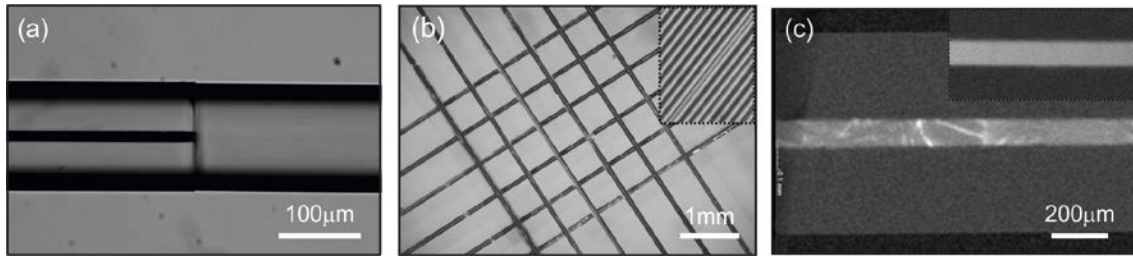
Figure 5. (a) Splicing of a silicon fibre to a conventional silica fibre. (b) A silicon fibre mesh (inset: dense stacking of silicon fibres). (c) X-ray tomography slice partway through a \text{Si}_{0.94}\text{Ge}_{0.06} alloy fibre showing composition fluctuations (inset: the uniform SiGe core after laser processing).
