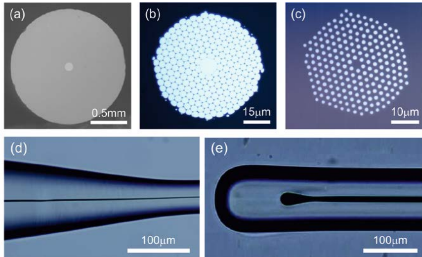
Figure 3. An assortment of silicon optical fibres. Microscope images of (a) a molten core derived step index fibre, and two HPCVD fabricated PCFs where (b) is an index guiding silicon core fibre and (c) is a bandgap guiding silica core fibre. Post-processed silicon fibres where in (d) the core is tapered longitudinally and (e) it is shaped to form a microspherical resonator at the end.
