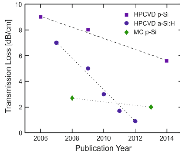
Figure 2. Year-on-year progress to reduce the losses in the silicon optical fibres fabricated by both the molten core (MC) and HPCVD approaches; dashed lines simply are a guide for the eye. Values are plotted for fibres both with polysilicon and hydrogenated amorphous silicon core materials, taken from the references: [6-8,13,16,24-27].
