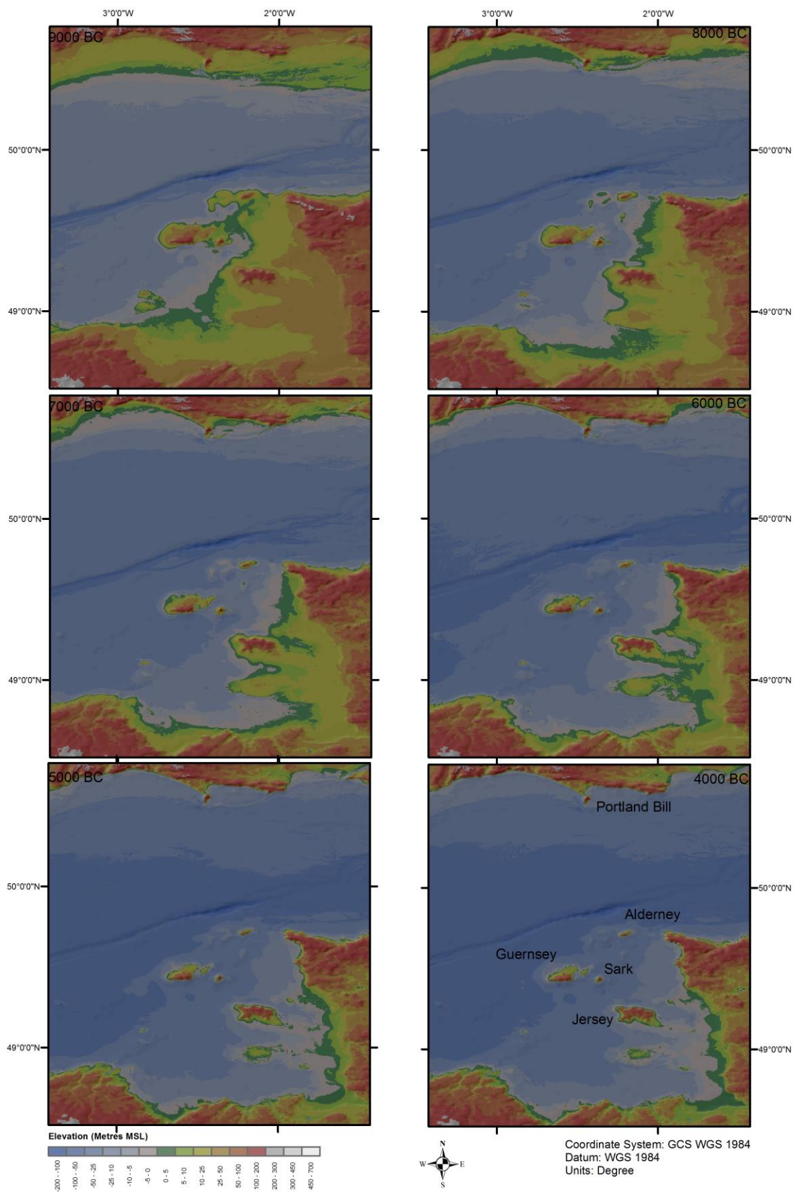
Figure 2. Graphical representation of sea-level and palaeogeographic change for the Channel Islands between 9000 and 4000 BC. Data from EMODnet ( www.emodnet.eu ) and GEBCO 2014 ( www.gebco.net )
