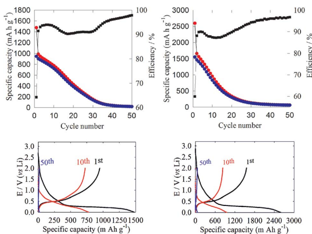
Fig. 6 Specific capacity versus cycle number (top), reduction blue, oxidation red and coulombic efficiency (black) and voltage profile against specific capacity (bottom), of Sn 3 N 4 /lithium half cells made with sodium alginate binder, cycled between 1 mV and 2 V for 50 cycles at 200 (left) or 100 (right) mA g -1 .
