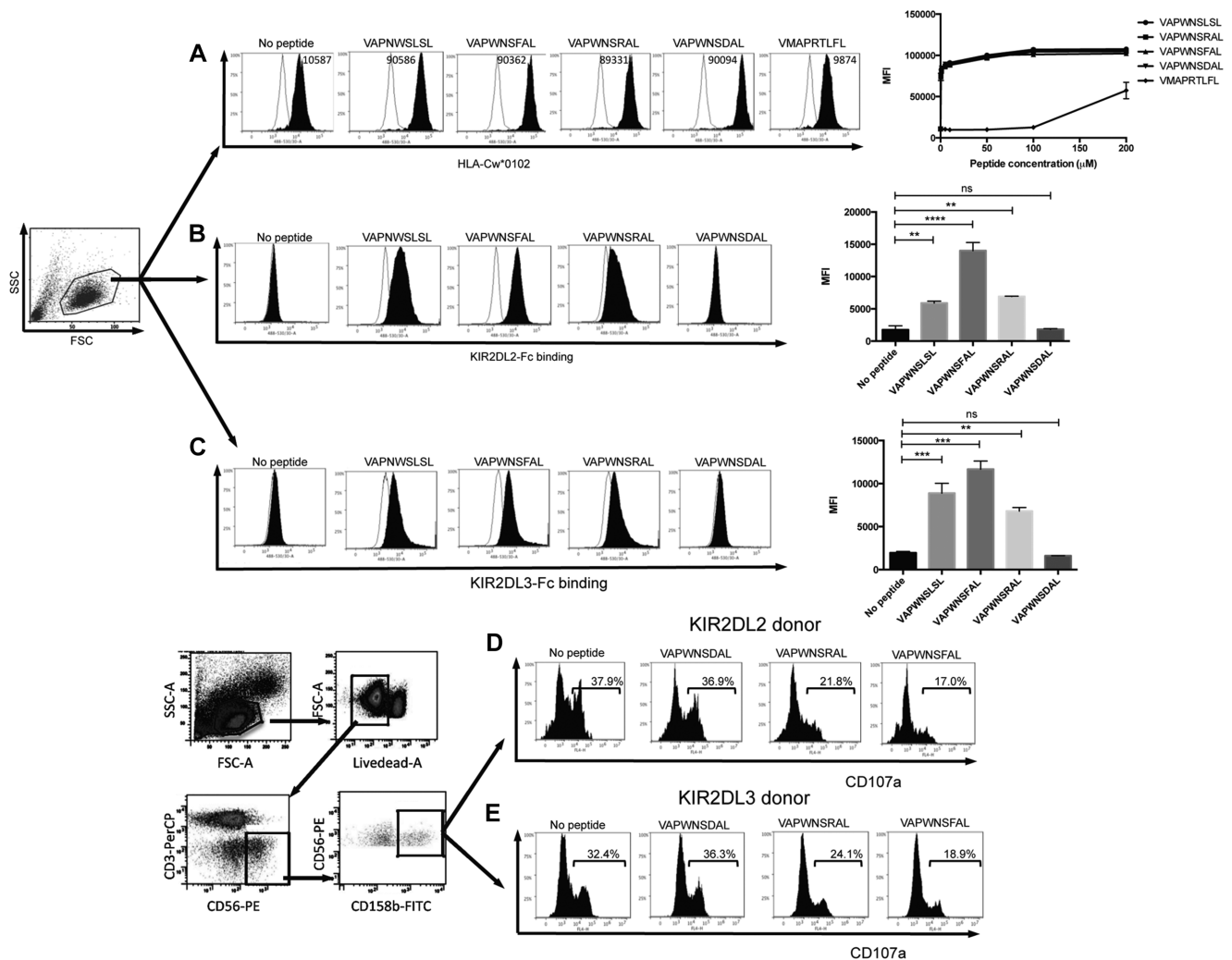
Figure 1. Correlation of KIR binding with NK cell inhibition in KIR2DL2+ and KIR2DL3+ donors. (A) Stabilization of HLA-Cw*0102 on 721.174 by the indicated VAPNWSLSL derivative peptides and a control peptide (VMAPRTLFL) at saturating concentrations 10 \mu M (filled histograms). The no primary Ab control is indicated in each plot and the titration of the peptides is shown in the far right panel. Binding of (B) KIR2DL2 or (C) KIR2DL3 fusion constructs to 721.174 cells in the presence (filled lines) or absence of the indicated peptide at a concentration of 10 \mu M. Representative histograms ( n = 3 samples) are shown. Summaries of the mean fluorescence intensities (MFI) of KIR-binding pooled from two independent experiments are shown in the far right panels (** p < 0.01 , *** p < 0.001 ; Student's t -test). Gating strategy and degranulation assays of CD158b-positive CD3-CD56+ NK cells from (D) KIR2DL2 homozygous or (E) KIR2DL3 homozygous donors in response to 721.174 cells incubated with the indicated peptides at a final concentration of 10 \mu M. Representative histograms of six 2DL2 and eight 2DL3 donors, analyzed in duplicate, are shown.
