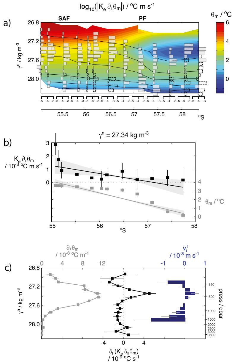
FIG. 7. (a) Meridional section along the JC69 occupation of the SR1b transect of K_e \partial_{\parallel} \theta_m . Positive (negative) values are indicated by gray (dashed) bars; \theta_m is shown by the background shading. Pressure contours are superimposed in black and labeled in Fig. 4a. Frontal positions are indicated in the upper axis. (b) Illustrative meridional distributions of \theta_m (gray squares) and K_e \partial_{\parallel} \theta_m (black squares) for the \gamma^n = 27.34 \text{ kg m}^{-3} isoneutral in the JC69 data. The lines (with shaded uncertainties) show the linear fits to the measured distributions, which are used to estimate section-characteristic gradients of both variables (see section 5). (c) Section-characteristic profiles of \partial_{\parallel} \theta_m , \partial_{\parallel}(K_e \partial_{\parallel} \theta_m) , and the contribution to \bar{v}^{\dagger} balanced by isoneutral stirring [only velocities corresponding to statistically significant values of \partial_{\parallel}(K_e \partial_{\parallel} \theta_m) are shown]. The section-mean pressure profile of isoneutral surfaces is indicated on the right-hand axis.
