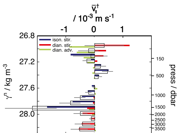
FIG. 10. Section-characteristic profile for the JC69 occupation of the SR1b transect of \bar{v}_{\perp}^t (open bars, with error bars), with contributions balanced by isoneutral stirring, dianeutral stirring, and dianeutral advection respectively indicated by blue, red, and green bars. The section-mean pressure profile of isoneutral surfaces is indicated on the right-hand axis.
