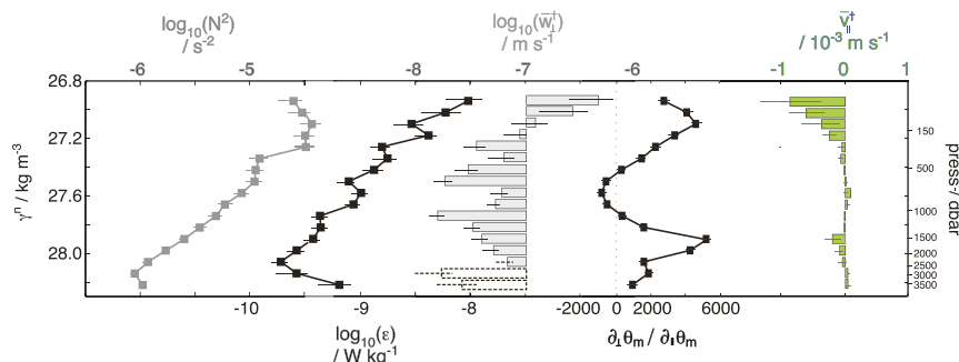
FIG. 9. Section-characteristic profiles of \log_{10}(N^2) , \log_{10}(\epsilon) , \log_{10}(\bar{w}_{\perp}^t) , \partial_{\perp}\theta_m/\partial_{\parallel}\theta_m , and the contribution to \bar{v}_{\perp}^t balanced by dianeutral advection of mean potential temperature. Negative values of \bar{w}_{\perp}^t are indicated by dashed bars. The section-mean pressure profile of isoneutral surfaces is indicated on the right-hand axis.
