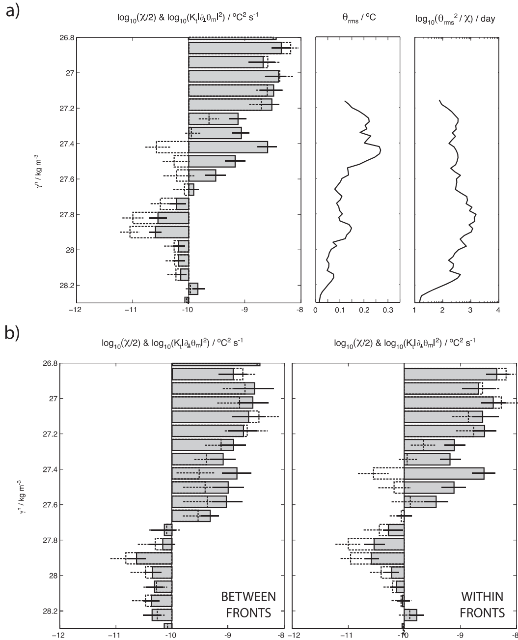
FIG. 5. (a) Mean profiles of (left) the rate of dissipation of temperature variance \chi/2 (gray bars) and the rate of dianeutral production of temperature variance K_t |\partial_\perp \theta_m|^2 (dashed bars), with uncertainties, for the JC69 occupation of the SR1b transect; (center) the rms potential temperature fluctuation in (10), estimated from all available SR1b hydrographic section repeats; and (right) the time scale of temperature variance dissipation, estimated as \theta_{\text{rms}}^2 / \chi using the data in the left and center panels. (b) As in (a), but partitioned into stations (left) between frontal jets and (right) within frontal jets; a station is defined to be within a frontal jet if the LADCP-measured speed exceeds 0.15 \text{ m s}^{-1} somewhere in the water column.
