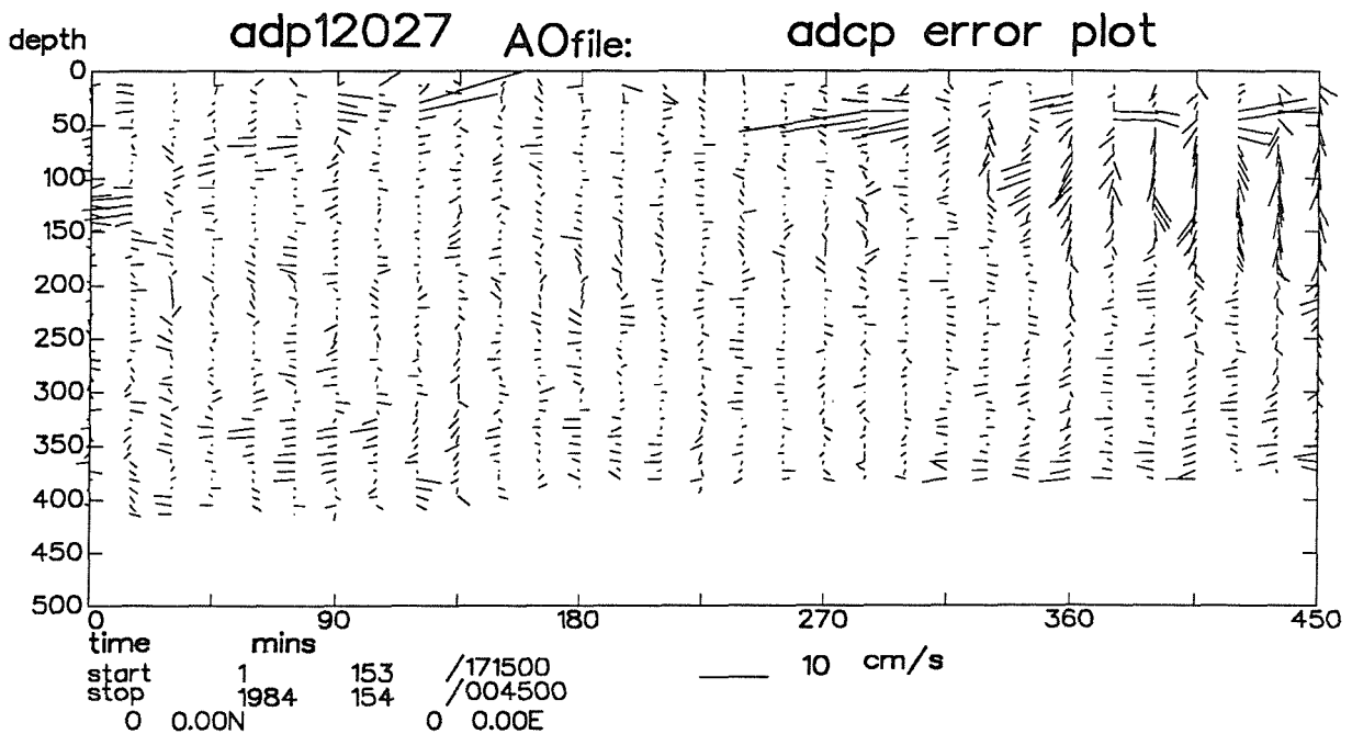
Figure 5 A pseudo-vector plot of vertical velocity (Y axis) and error velocity (X axis). Normally noise like, coherent areas such as after T=350 minutes, and around a depth of 50 metres, indicate interference. The likely cause in this on-station period was scatter from the CTD wire.
