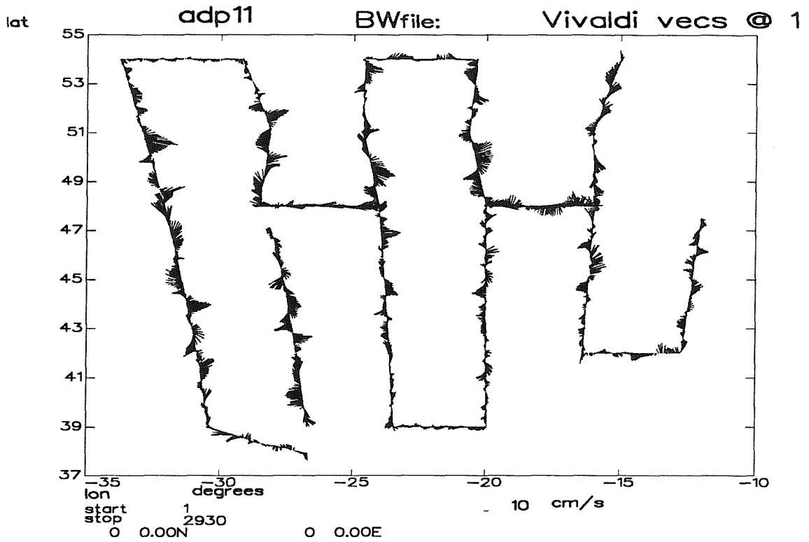
Figure 7 Current vectors whilst underway from a depth of 101 metres, every 4km, along the Vivaldi '91 cruise track. Note that eddies, eg on the western leg, are well resolved.
