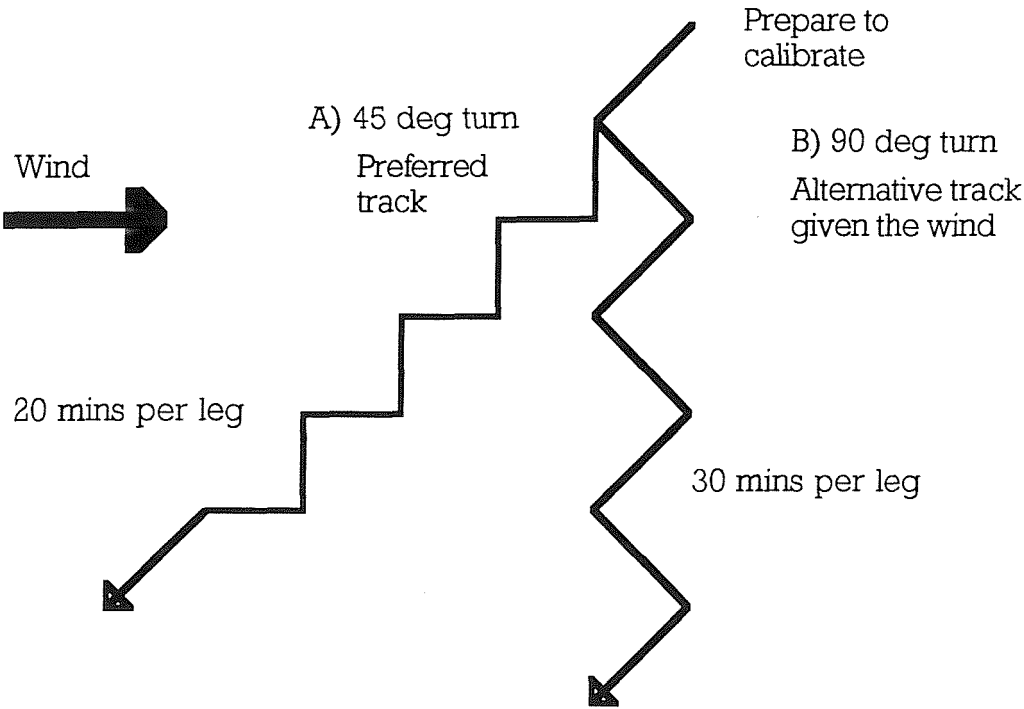
Figure 2 Example ADCP calibration track, showing the preferred track and an alternative if there is significant wind.
