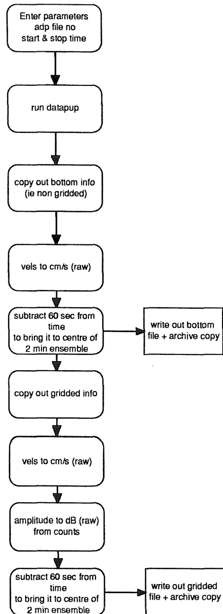
Flow chart for the script adpexec0
