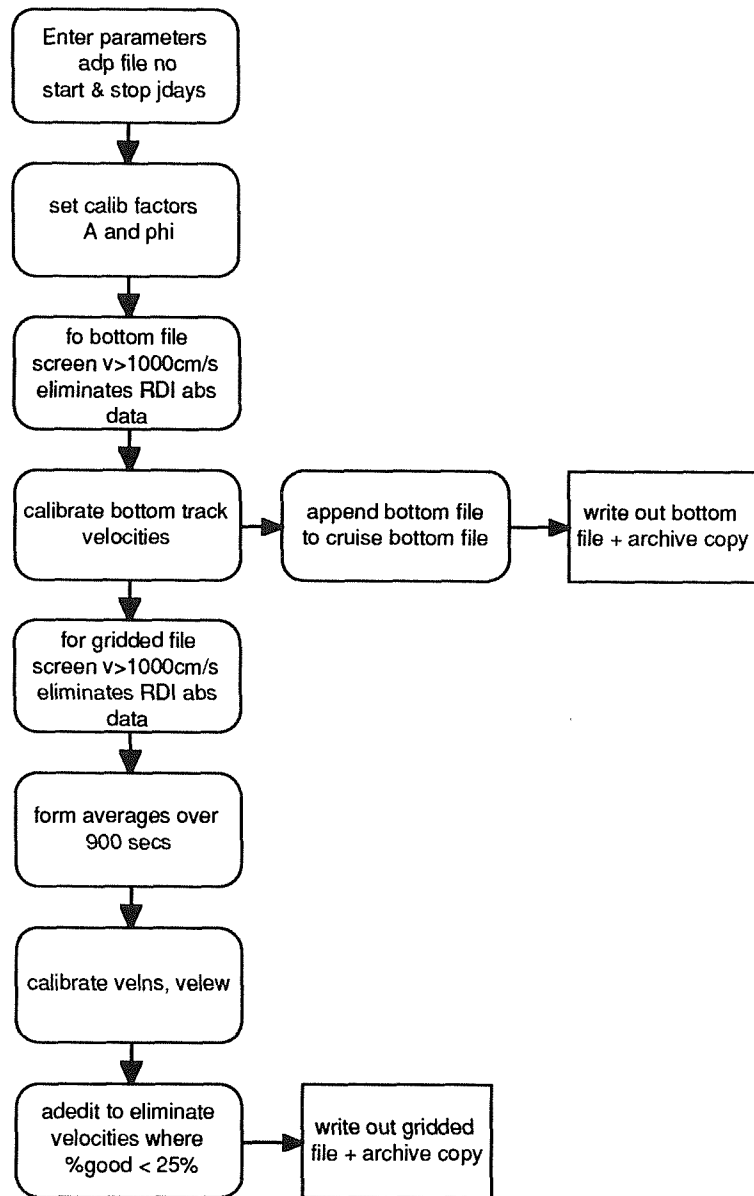
Flow chart for the script adpexec2
