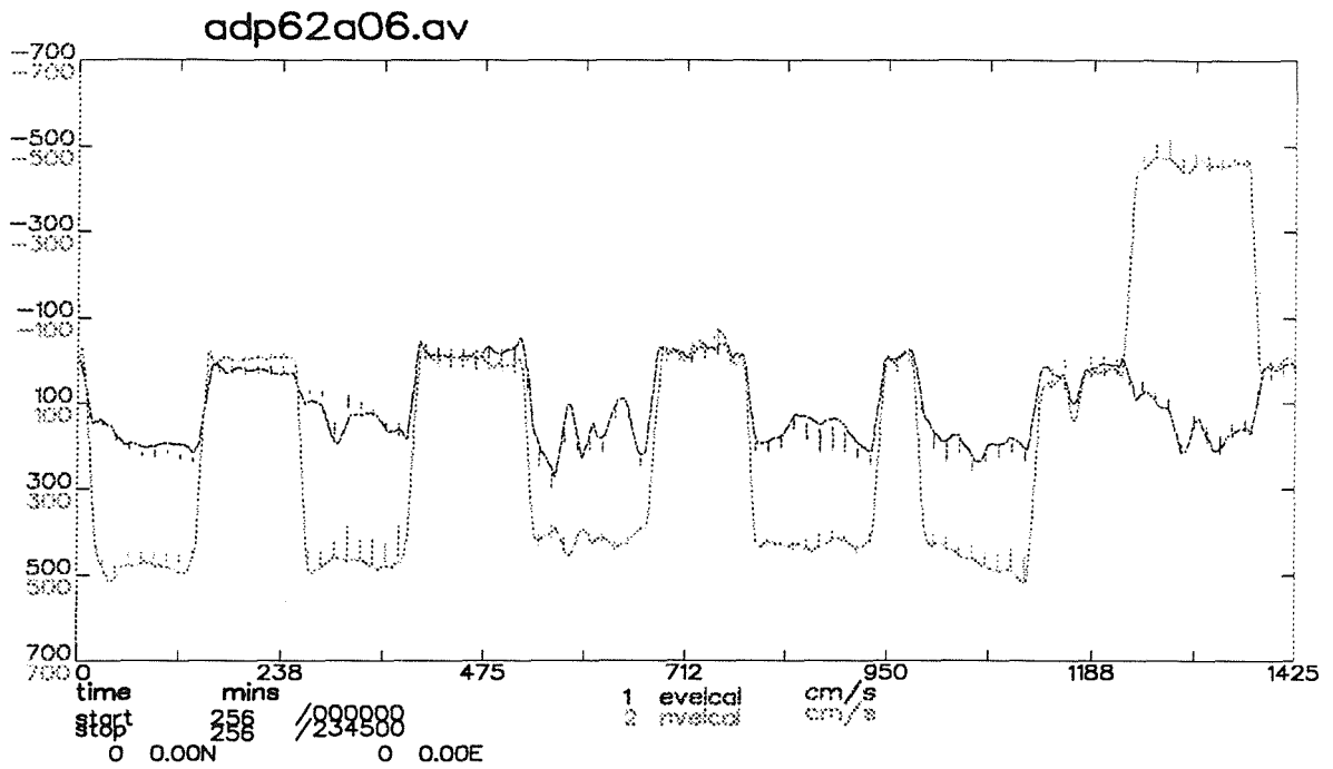
Figure 4 Comparison of ship velocity over the ground obtained by GPS (solid lines) and ship velocity through the water from the ADCP (vertical bars). This form of plot is useful for pinpointing poor profile data or poor navigation data.
