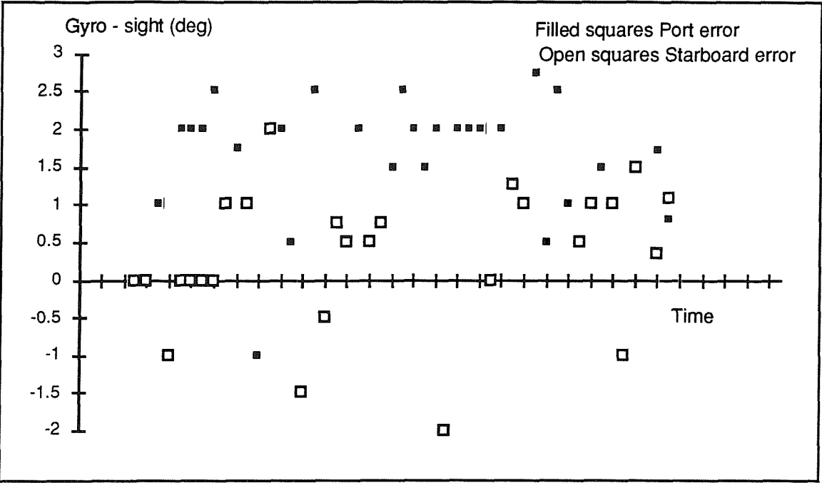
Figure 1 Example of a Gyro - star sight time series during the six weeks of Vivaldi '91, for the port and starboard repeaters.
