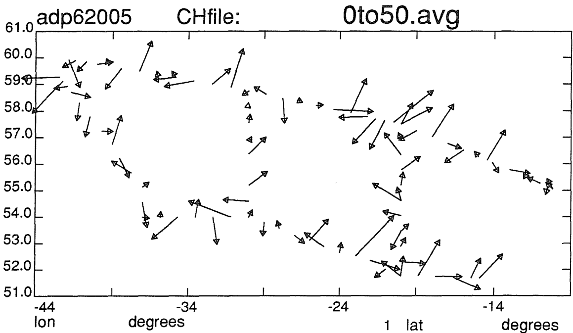
Figure 8 Horizontal map of mean 'on-station' current vectors averaged over the depth range 0 to 50 metres from CONVEX '91. The program allav was used to obtain the vectors, and they were plotted using the program vecplo. The scale is 0.3mm to 1 cm/s.
