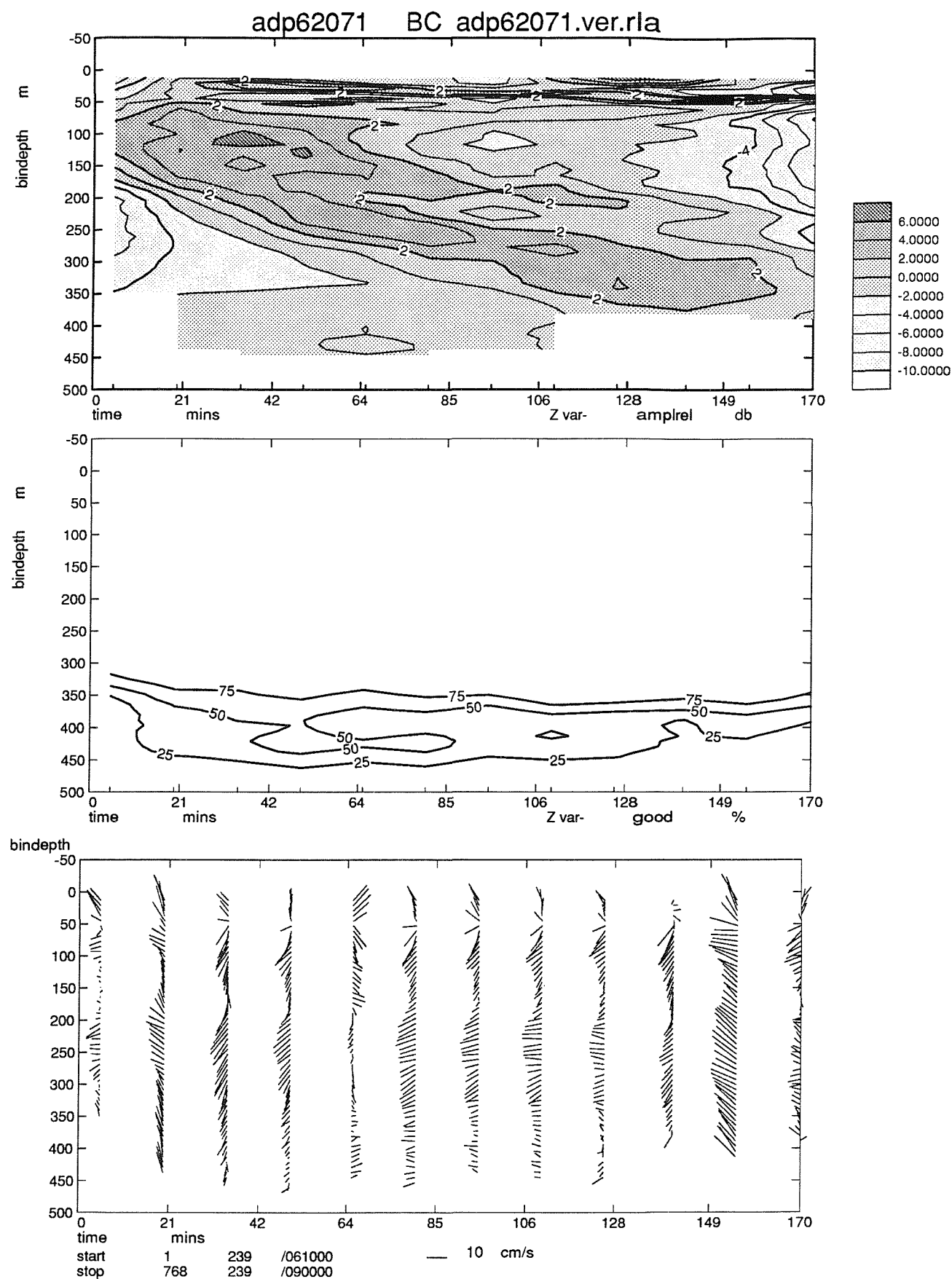
Figure 6 Example plots taken from Charles Darwin cruise 62 (CONVEX) whilst on station; they show relative amplitude (top), %good (centre) and absolute current vectors (bottom). The relative amplitude plot is an example of dawn downward migration of zooplankton. The %good plot shows good data down to 350 metres. The vector plot shows a different current structure in the upper 50 metres to that prevalent beneath. Much of the variation between profiles is because of errors in the ship velocity inferred from GPS navigation. This page was generated using the scripts preport and adppage1.
