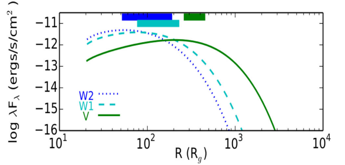
Figure 10. Disc emissivity profile in W2, W1 and V bands (lines) for the parameters given in the text, with measured lags, relative to the X-ray bands, as bars at the top. The W1 bar lies below the W2 and V band bars.
