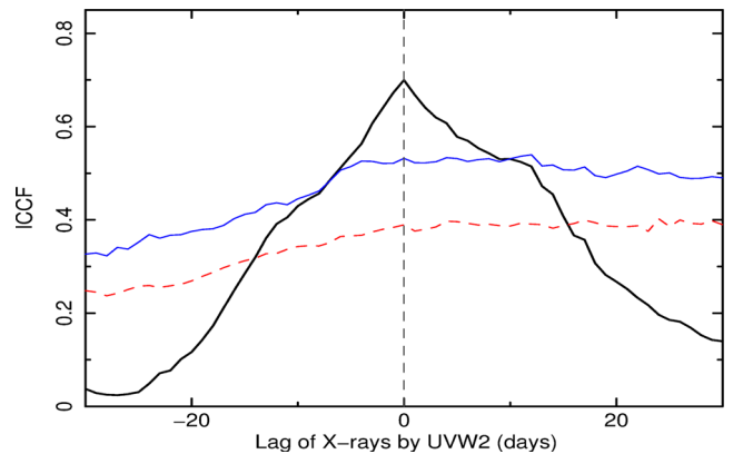
Figure 4. Interpolation cross-correlation function between the X-ray and UVW2 light curves shown in Fig. 1. The 95 per cent (dashed red) and 99 per cent (thin blue) confidence levels are also shown.
