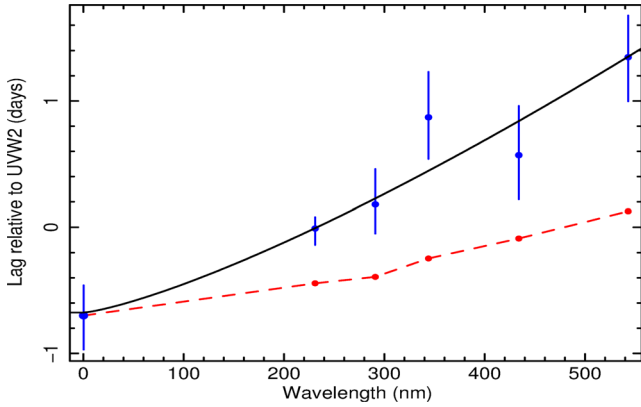
Figure 9. Lag of the X-ray and other UVOT bands relative to UVW2. \text{Lag} \propto \text{wavelength}^\beta , where \beta = 1.23 \pm 0.31 . The lower, dashed, red line is the prediction for a standard disc as described in the text.
