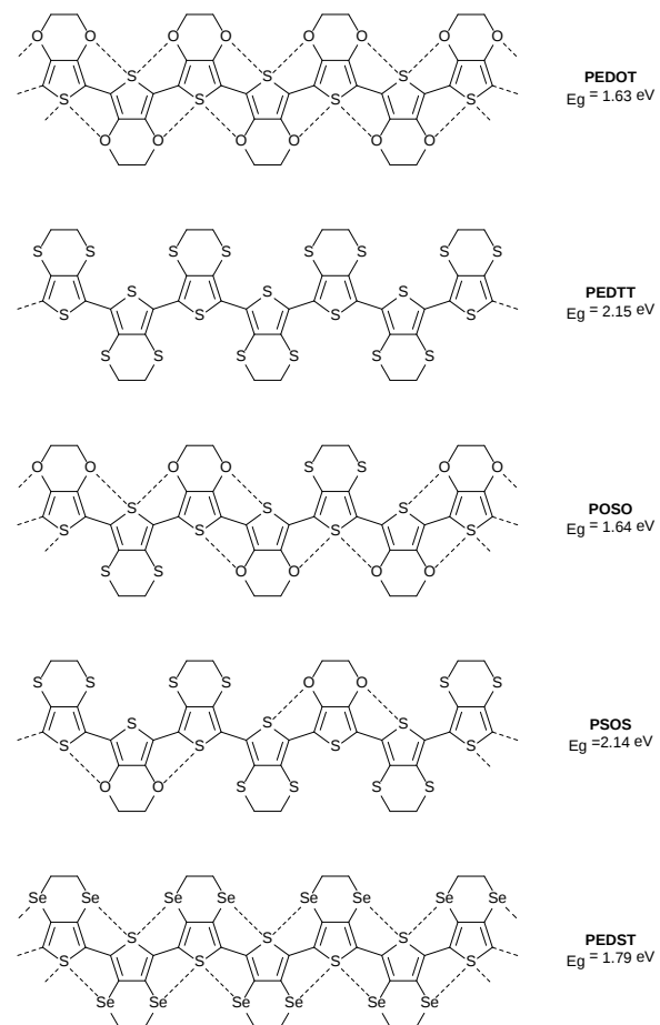
Figure 2. Chemical structure of the polymer PEDOT and its chalcogen variants, showing non-covalent interactions as dashed lines. The corresponding band gaps are given in eV.
