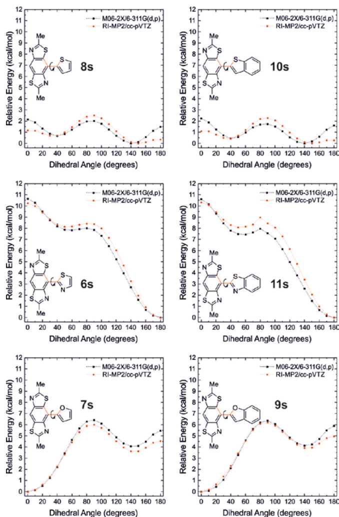
Figure 6. Torsional potential surfaces for fragments of 6-11 calculated at the M06-2X/6-311G** (black) and RI-MP2/cc-pVTZ (red) levels of theory. Rotation occurs around the inter-ring C-C bond marked in red, starting from the conformation shown (0°).
