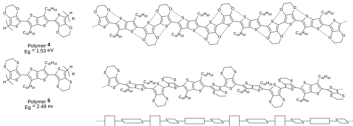
Figure 3. Structures of polymers 4 and 5 with the twisted conformation of 5 in schematic form shown on the bottom.
