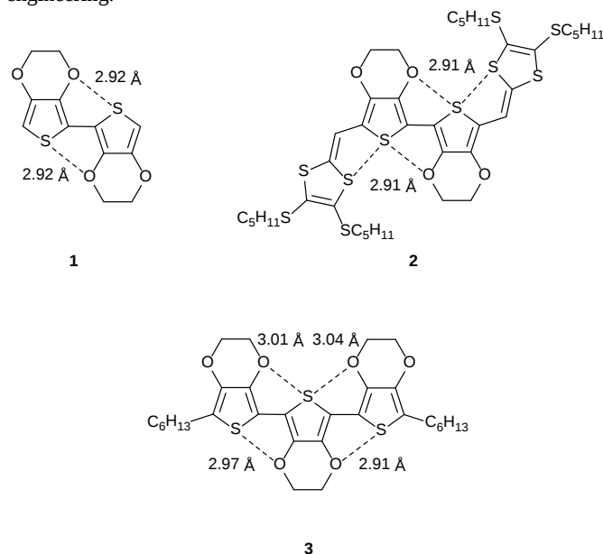
Figure 1. Compounds 1-3 showing short contact distances between heteroatoms.
