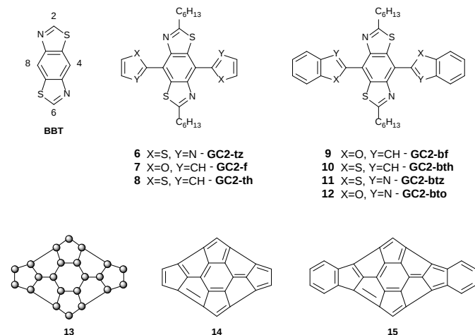
Figure 4. Substitution pattern of BBT, target compounds 6-12 and hypothetical structures 13-15 .
