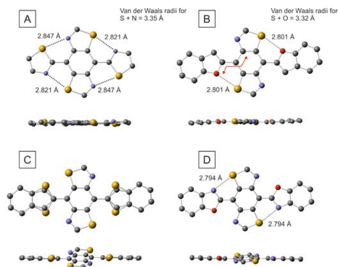
Figure 5. Molecular structures of compounds 6 (A), 9 (B), 10 (C) and 12 (D), determined by single crystal X-ray diffractometry. The hexyl chains have been omitted for clarity. Close contacts between S-N and S-O are given as dashed lines.
