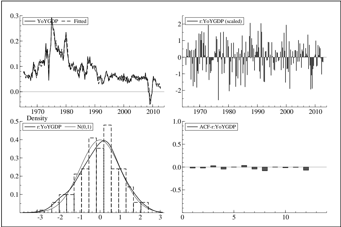
Figure 4: GUM 1 Diagnostic test plots
