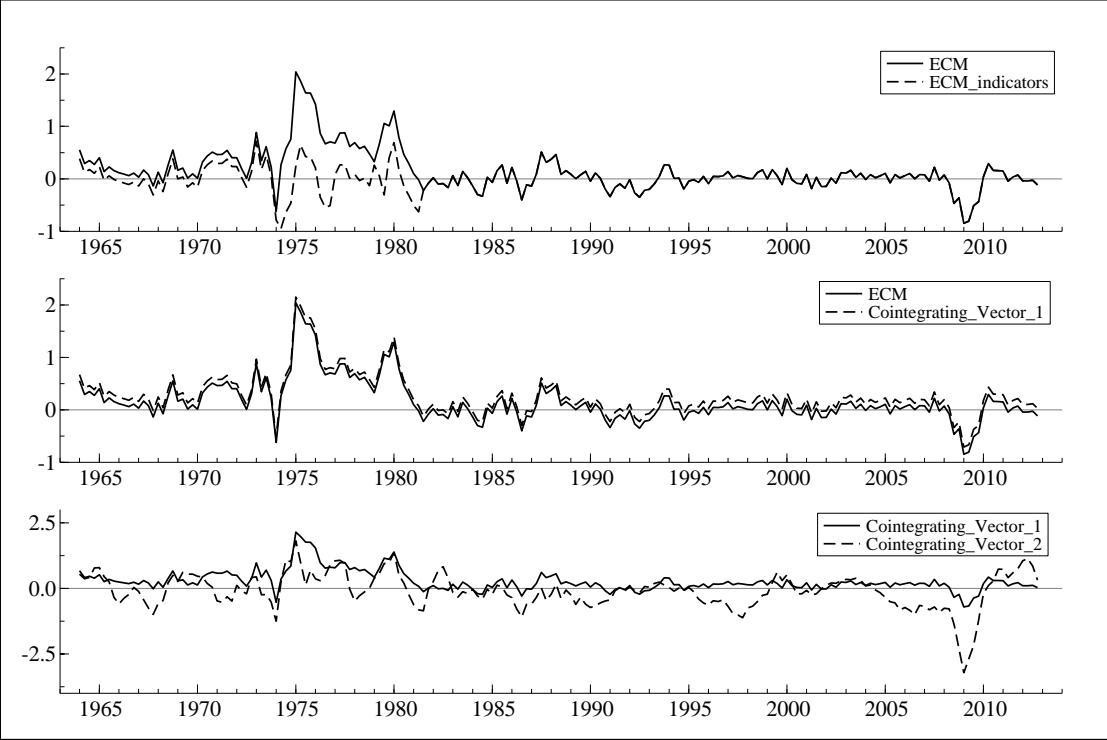
Figure 5: Error Correction and Cointegrating Vector plots
