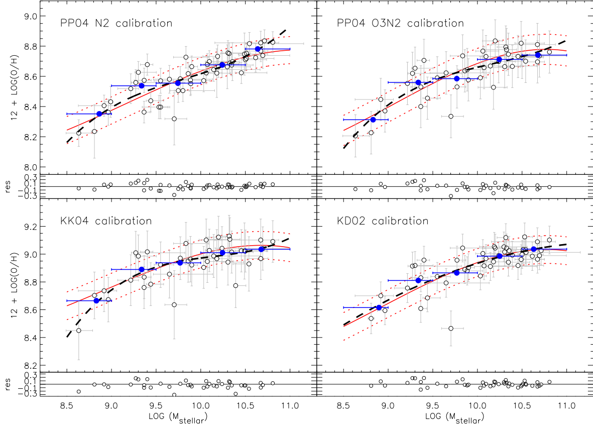
Figure 16. The metallicity-mass relations compared by different metallicity calibrations. Upper panels: PP04 N2 (left) and PP04 O3N2 (right) calibrations. Lower panels: KK04 (left) and KD02 (right) calibrations. The open circles show the measurements in this work. The blue filled-circle is the mean metallicity in bins of M_{\text{stellar}} . The best fit to field galaxies given by Kewley & Ellison (2008) with the range of one r.m.s. scatter was over-plotted (in red line and red dashed-line, respectively). The black dashed-line is the best fit to the measurements in this work. The sub-plot in the bottom of each panel represents the residuals of our measurements from KE08's best fit.
