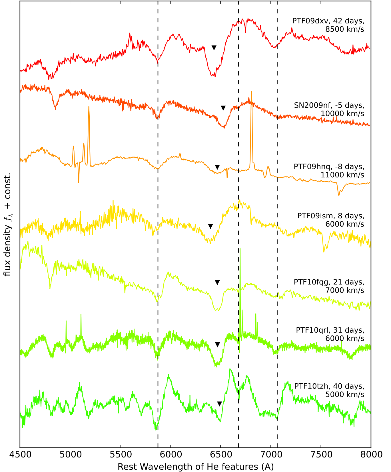
FIG. 8.— Representative spectra of the PTF-detected SNe in our sample. All spectra are redshifted by the indicated velocity relative to the rest frame such that their characteristic helium absorption features are at their rest wavelengths at 5876 Å, 6678 Å, and 7065 Å (indicated by broken lines). In addition, the black triangles mark the prominent H \alpha absorption lines. The H \alpha emission line is found to the right of these features and often has a flat-top profile owing to the helium absorption at 6678 Å. Some SNe are compared to known SNe IIB identified with SNID (Blondin & Tonry 2007) and the time after peak is indicated next to all spectra. All spectra are available electronically via the WISEREP webpage (Yaron & Gal-Yam 2012). Further spectra are shown in Figures 9 and 10.
