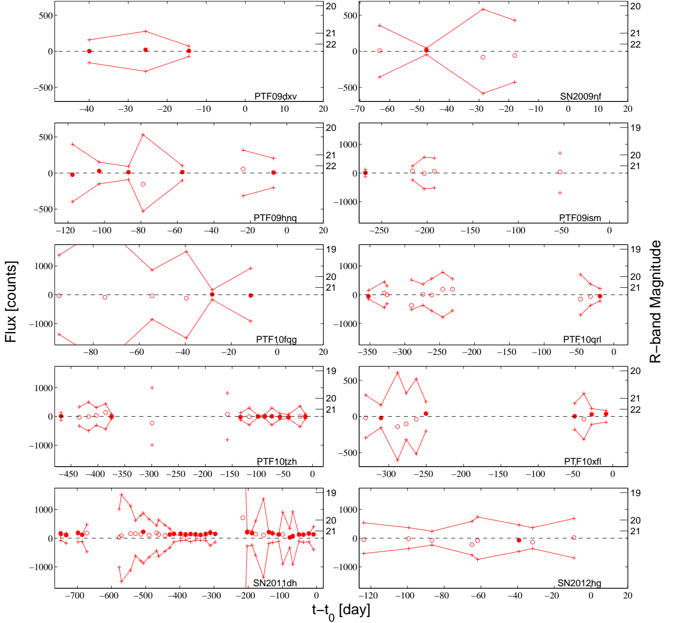
FIG. 1.— The pre-explosion light curves of the first ten SNe (names are listed in each panel; compare Table 1). Shown are flux residuals (relative to the reference image given in counts per 60 s exposure) coadded in 15-day bins prior to the SN explosion. The right-hand axis shows apparent m_{PTF,R} -band magnitudes. All measurements are in the PTF magnitude system (Ofek et al. 2012a,b). The zero point of the flux residuals is 27. Filled circles represent 15-day bins with six or more observations and open circles mark bins having less data. The plus signs show the 5\sigma noise level, which is estimated based on scaled Poisson errors for the open circles and with the bootstrap method (Efron 1982) for filled circles (see §4.1 for a detailed description). If observations are found in consecutive bins, the plus signs are connected by a solid line. A few very large error regions are outside the plotted range to improve readability. Figures 2 and 3 show the pre-explosion light curves of the remaining SNe.
