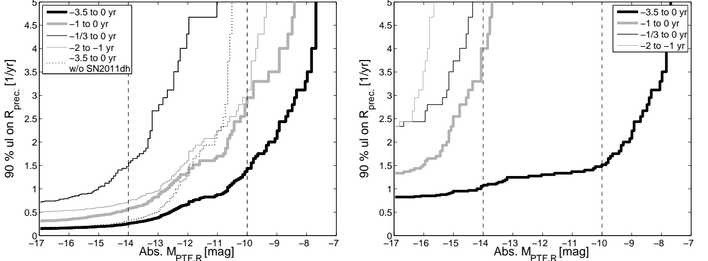
(a) 90% upper limit on precursor rate derived from the complete SN I Ib sample (b) 90% upper limit on precursor rate derived from five double-peaked SNe I Ib
