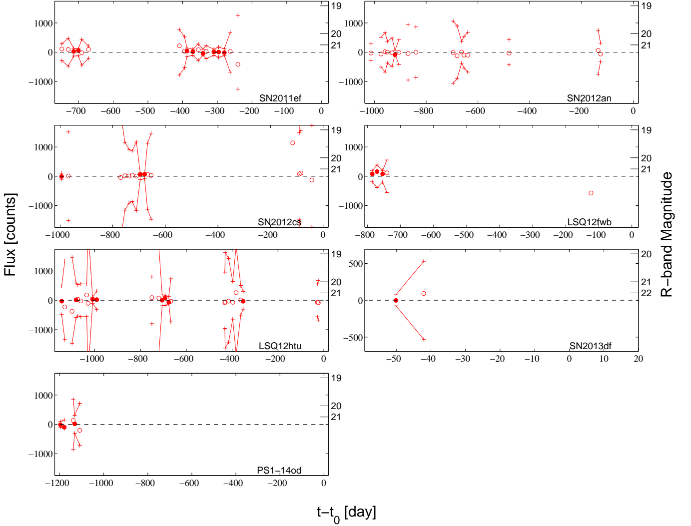
FIG. 3.— Figures 1 and 2, continued. Here we show the PTF pre-explosion light curves of SNe IIb found in the literature.
