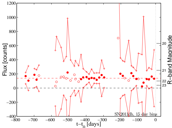
FIG. 5.— The binned pre-explosion light curve of SN 2011dh. The reference images are chosen to be after the explosion, hence the flux of the progenitor has not been subtracted. No observations deviate by more than 5\sigma from the mean flux.
