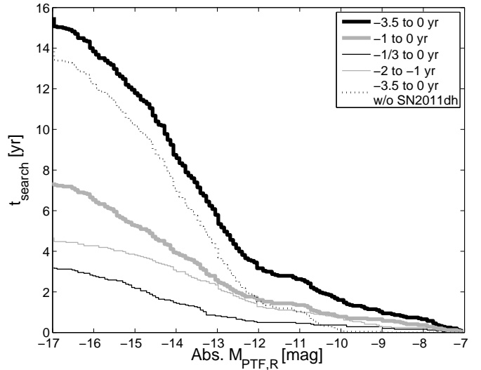
FIG. 6.— The absolute-magnitude dependent control time for the complete sample, during which the SN locations were observed and no precursors were detected above the given magnitude. The various curves are for precursors taking place at different time ranges prior to the SN explosion (see legend). The curve normalization and shape are determined by the amount of data and the SN distances. SN 2011dh accounts for most observations at the brightest magnitudes and the dotted line shows the effect of removing it from the sample. Additional curves display the control time for shorter periods before the explosion. The limiting magnitudes per bin for all SNe are listed in Table 4.
