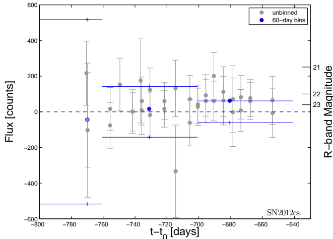
FIG. 4.— A section of the pre-explosion light curve of SN2012cs. The gray error bars show the scaled up 1\sigma Poisson errors on the individual observations. The blue lines indicate the bin position as well as the 5\sigma noise level for the binned light curves. Open dots represent bins containing fewer than 6 observations for which the noise level is estimated based on the scaled Poisson errors. Filled dots correspond to bins with at least 6 observations and the bootstrap method was used to estimate the noise level. A detection, marginally above the 5\sigma threshold, is obtained around day -680 . The false alarm probability of SN2012cs is 1.8% when using 60 day bins.
