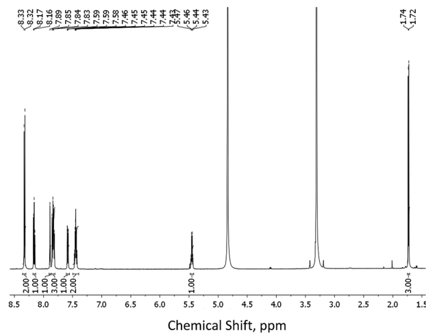
Fig. 1 ^1\text{H} NMR of \mathbf{1(S)} (600 MHz, \text{CD}_3\text{OD} ).
