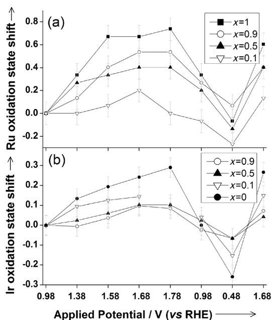
Figure 5. Plots of shifts in oxidation states of a) Ru and b) Ir derived from analysis of the in situ XANES spectra measured during electrochemistry of (\text{Na}_{0.33}\text{Ce}_{0.67})_2(\text{Ir}_{1-x}\text{Ru}_x)_2\text{O}_7 materials. Note that in (b) one data point is missing for the x=0.1 material due to interference from evolved oxygen bubbles.
