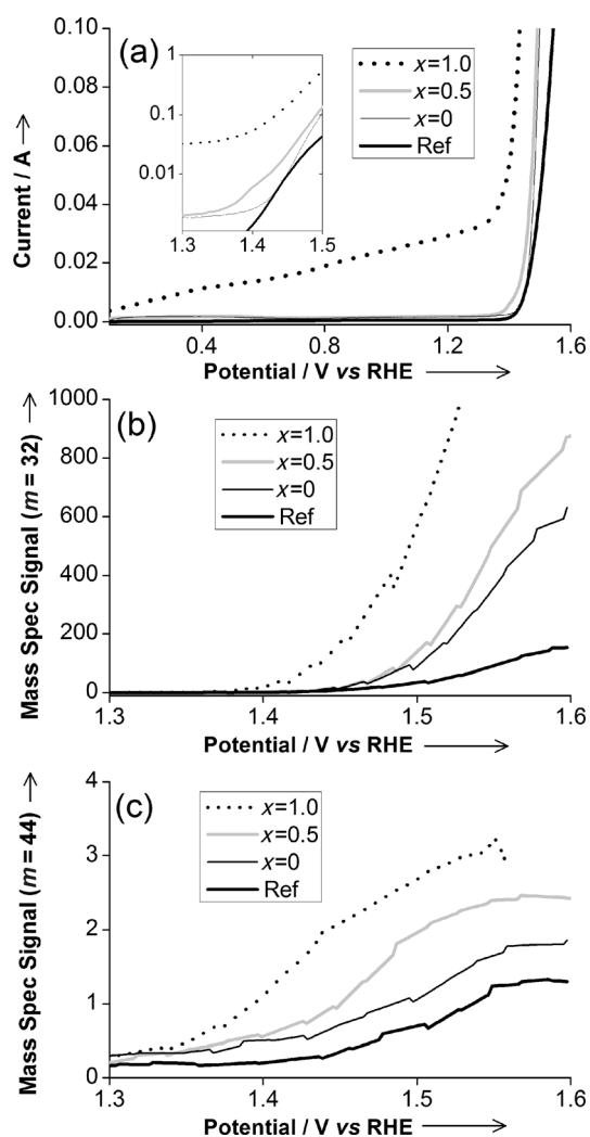
Figure 3. Differential electrochemical mass spectroscopy of (\text{Na}_{0.33}\text{Ce}_{0.67})_2(\text{Ir}_{1-x}\text{Ru}_x)_2\text{O}_7 pyrochlores and reference Ru-Ir rutile oxide (\text{Ru}_{0.9}\text{Ir}_{0.1})\text{O}_2 (Ref) during 10\text{ mVs}^{-1} potential sweep showing: a) current response, b) oxygen evolution, c) \text{CO}_2 evolution (competing carbon corrosion).
