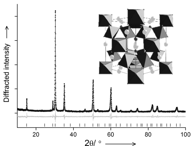
Figure 1. Refined powder X-ray diffraction pattern ( \lambda = 1.5406 \text{ \AA} ) of (\text{Na}_{0.33}\text{Ce}_{0.67})_2(\text{Ir}_{0.5}\text{Ru}_{0.5})_2\text{O}_7 . The line is the fitted profile, black points the measured data, the pale line the difference and the ticks the positions of allowed Bragg reflections ( Fd\bar{3}m , a = 10.2242(3) \text{ \AA} ). The inset is a view of the \text{A}_2\text{B}_2\text{O}_6\text{O}' pyrochlore (B-site octahedra, light grey A-site and dark grey O').
