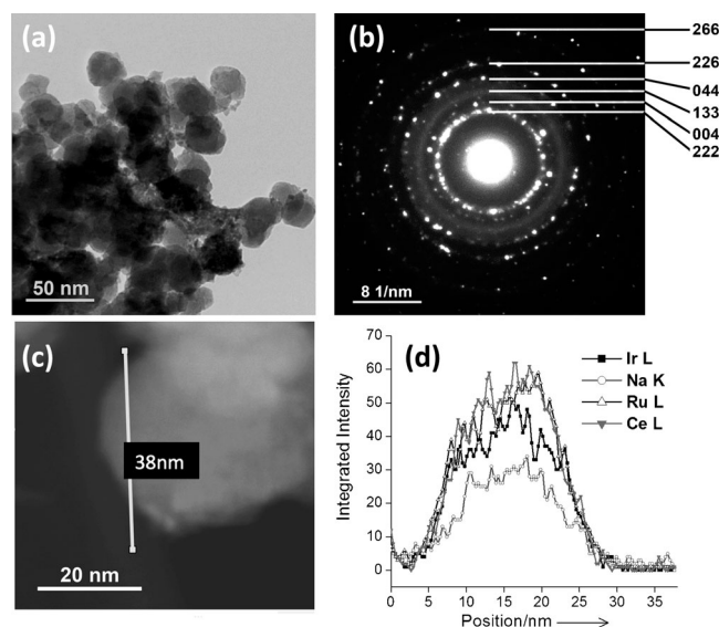
Figure 2. TEM analysis of (\text{Na}_{0.33}\text{Ce}_{0.67})_2(\text{Ir}_{0.5}\text{Ru}_{0.5})_2\text{O}_7 nanoparticles; a) image of a typical region of specimen; b) SAED of agglomerated nanocrystals in (a) indexed using the F-cubic pyrochlore unit cell from XRD; c) representative single particle with the line profile region for the linear analysis in (d) indicated, and d) results of a typical EDXA line-scan analysis of particle in (c). Further EDXA lines scans are presented in the SI.
