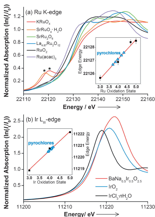
Figure 4. XANES spectra at a) Ru K edge [ \text{Ru}^{(+3)} (acetylacetonate) _3 , \text{Ru}^{(+4)}\text{O}_2 , \text{La}_{4.87}\text{Ru}^{(+4.70)}_2\text{O}_{12} , \text{SrRu}^{(+5)}_2\text{O}_6 , \text{SrRu}^{(+6)}\text{O}_4 \cdot \text{H}_2\text{O} , and \text{KRu}^{(+7)}\text{O}_4 ] and b) Ir L_{\text{III}} edge ( \text{Ir}^{(+3)}\text{Cl}_3 \cdot n\text{H}_2\text{O} , \text{Ir}^{(+4)}\text{O}_2 , and \text{BaNa}_{0.5}\text{Ir}^{(+5)}_{0.5}\text{O}_{2.5} ). In (a) the 1s–4d transition of \text{KRuO}_4 and \text{SrRuO}_4 \cdot \text{H}_2\text{O} is indicated by *. Insets show graphs of edge position versus oxidation state with the blue triangles for the pyrochlores giving the average oxidation state of +4.00 and +4.05 for Ru and Ir, respectively.
