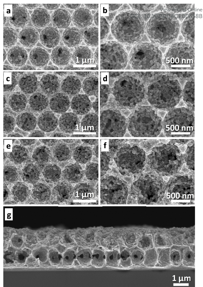
Fig. 6. (a-f) Top view SEM images at low and high magnifications showing the MOF products formed on the walls of the ordered macroporous Cu electrodes (3/2 layers of pores), via the oxidation at 0.125 V for various reaction times (a-b) 30 s, (c-d) 60 s and (e-f) 120 s in a solution of 0.05 M BTC in ethanol containing 0.2 M MTBS supporting electrolyte. (g) Typical cross sectional image obtained for the 60s samples.
