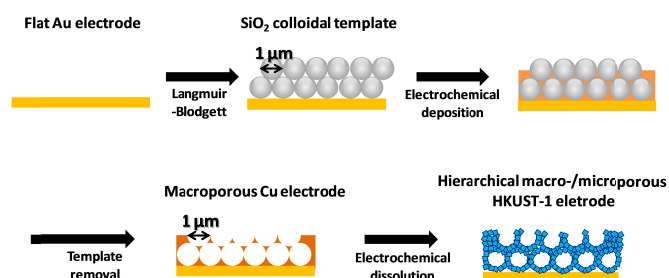
Scheme 1. Schematic illustration showing the experimental steps performed in this work for the synthesis of the hierarchical macro-/microporous HKUST-1.
