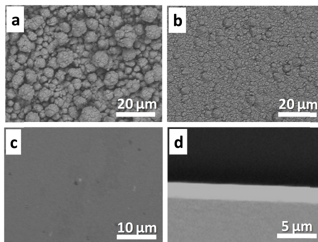
Fig. 1. Typical SEM images showing (a-c) the top-surface and (d) a cross-section of the Cu deposit using a Cu plating bath (CUBRAC 660) at various potentials: (a) -0.35, (b) -0.25 and (c-d) -0.05 V. The deposition time was 300 s.
