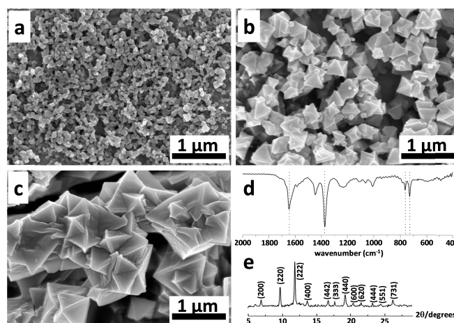
Fig. 4. (a-c) SEM images showing the MOF products formed on flat Cu surfaces via its electrochemical dissolution at 0.5 V for various times: (a) 60, (b) 600 and (c) 1800 s in a solution of 0.05 M BTC in ethanol containing 0.2 M MTBS supporting electrolyte. (d) FTIR and (e) XRD patterns recorded with the 1800s sample confirming the HKUST-1 structure.
