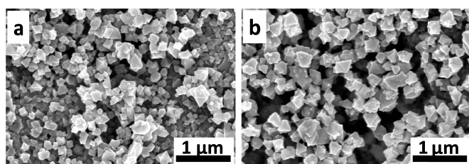
Fig. 3. SEM images showing the MOF products formed on flat Cu surfaces via electrochemical dissolution for different potentials, (a) 0.125 and (b) 0.5 V, but using the same reaction time (300 s) in a solution of 0.05 M BTC in ethanol containing 0.2 M MTBS supporting electrolyte.
