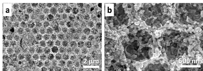
Fig. 5. (a) Low and high-magnification SEM images showing the top view of the macroporous Cu electrodes with 3/2 layers of pores after the MOF formation at a constant oxidation potential of 0.5 V and a reaction time of 60 s in a solution of 0.05 M BTC in ethanol containing 0.2 M MTBS supporting electrolyte.
