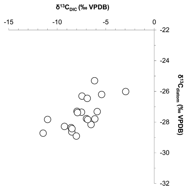
Figure 4. Significant positive relationship between \delta^{13}\text{C}_{\text{DIC}} and \delta^{13}\text{C}_{\text{diatom}} values determined for the contemporary UK river data set ( r_s=0.70 , P<0.01 ). Relationship identified using Spearman's rank correlation coefficient.
