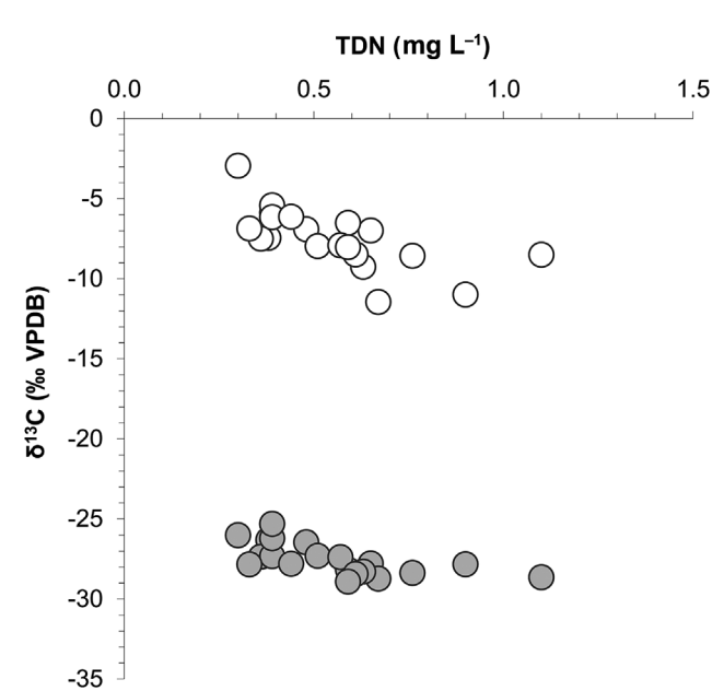
Figure 5. Significant negative relationships between TDN concentrations and \delta^{13}\text{C}_{\text{DIC}} (open circles) ( r_s=-0.77 , P<0.01 ) and \delta^{13}\text{C}_{\text{diatom}} (shaded circles) ( r_s=-0.73 , P<0.01 ) values determined for the contemporary UK river data set. Relationships identified using Spearman's rank correlation coefficient.
