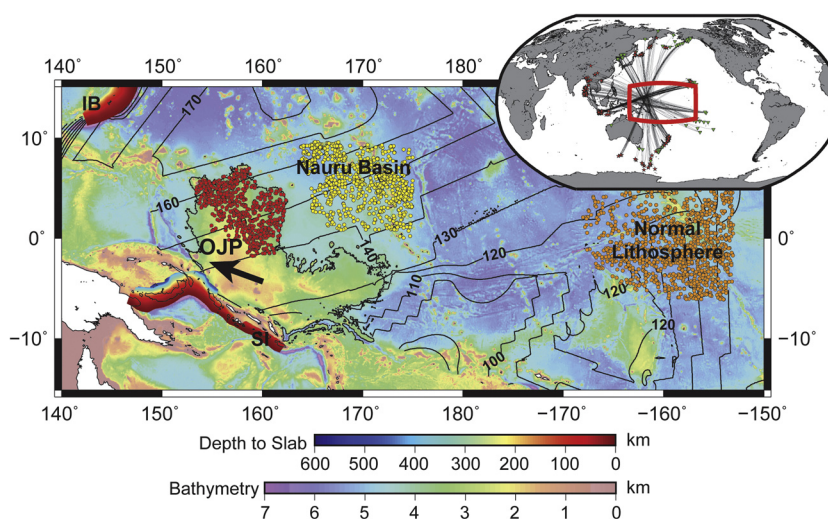
Fig. 1. Bathymetry map of the western Pacific with Ontong – Java Plateau (OJP) marked by 4000 m isobath. Colored circles show bouncepoints beneath OJP (red), Nauru basin (yellow) and normal oceanic lithosphere (orange) (Korenaga and Korenaga, 2008). Colored overlays labeled SI and IB show subducted slabs (Hayes et al., 2012) along the Solomon Islands (SI) and the Izu–Bonin–Mariana trench (IB). Background colors show bathymetry and contours represent the age of seafloor in My (Muller et al., 2013). Black arrow shows the present plate motion direction. Overlay global map shows the study region (red box) and event (red star)–station (green inverted triangle) pairs that have bouncepoints beneath OJP.
