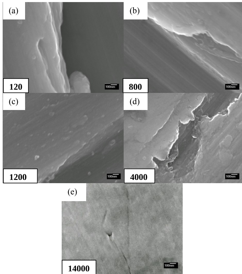
Figure 4 SEM images of CG sample substrates processed by (a) 120, (b) 800, (c) 1200 and (d) 4000 grit abrasive paper. (e) Surface polished by 14000 grit diamond paste before anodization.
