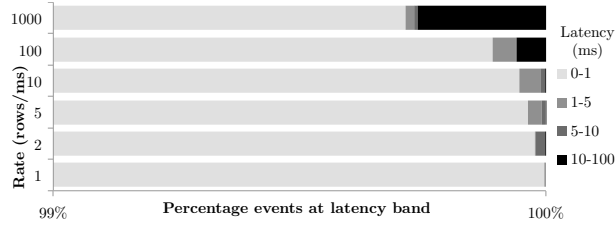
Fig. 4. Percentage Latency at Various Rates
