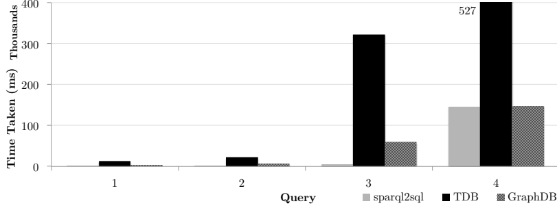
Fig. 3. Average Time Taken for Smarthome Analytical Queries
