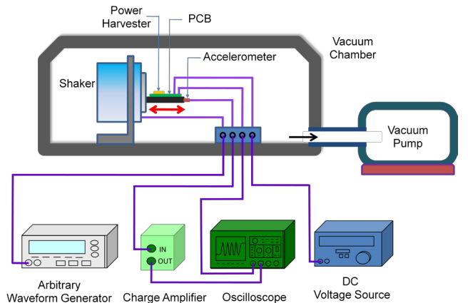
Fig. 7: Illustration of measurement setup.
