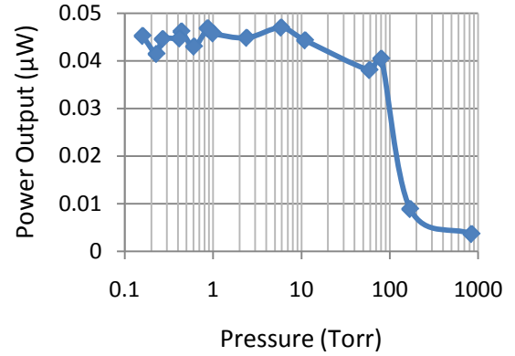
Fig. 11: Effect of pressure on output power.
