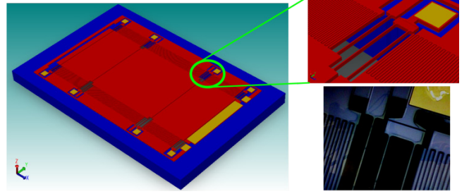
Fig. 5: 3DOF EPH showing the suspension and electrodes in both schematic and optical micrograph.
