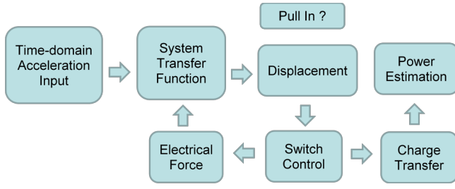
Fig. 3: Flow of the numerical system-level model.
