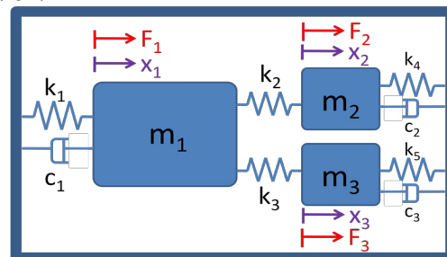
Fig. 1: A 3DOF spring-mass-damper system.
