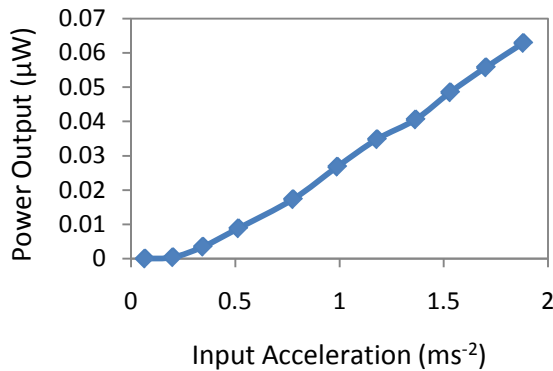
Fig. 9: Plot of output power versus input acceleration.
