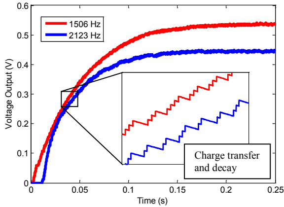
Fig. 4: Simulated output voltage at load resistor.
