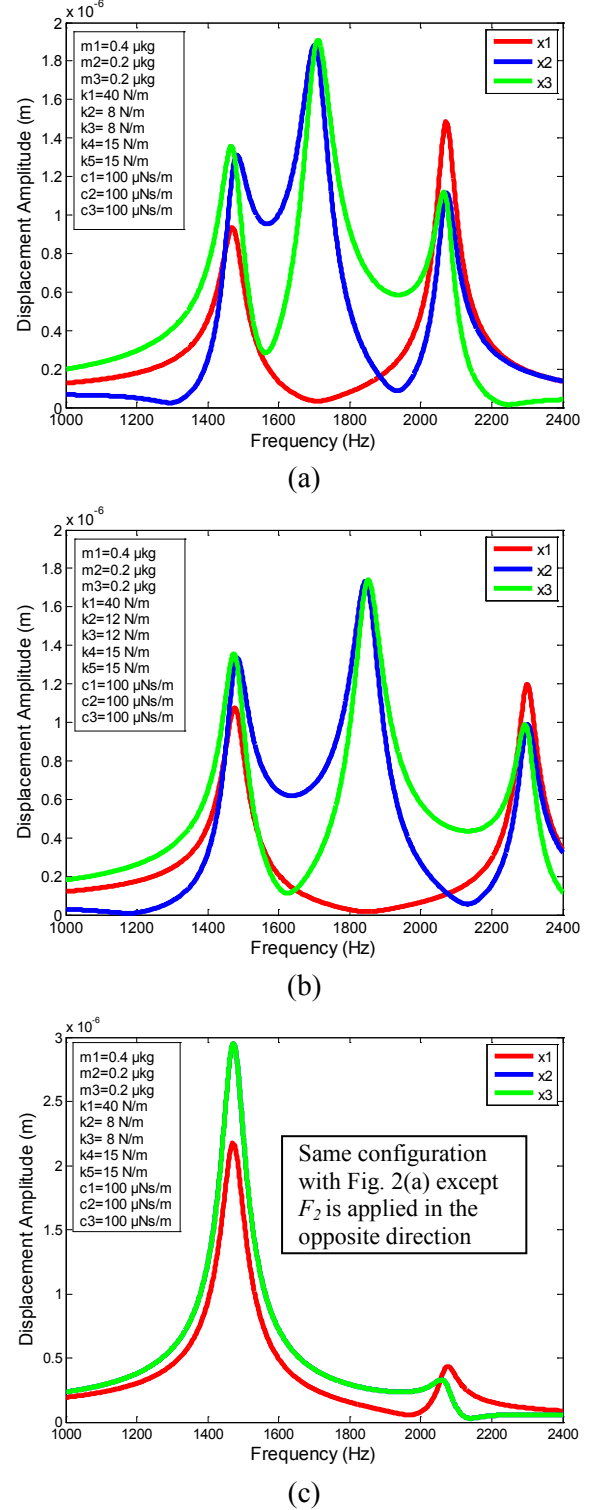
Fig. 2: Forced response of 3DOF system with different design parameters.
