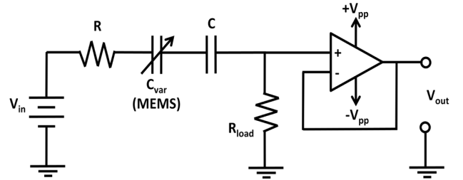
Fig. 6: Electrical measurement circuit.
