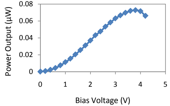
Fig. 10: Effect of DC bias voltage on output power.
