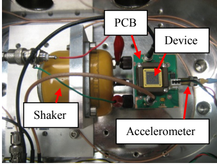
Fig. 8: A photograph of the test setup in a custom vacuum chamber.
