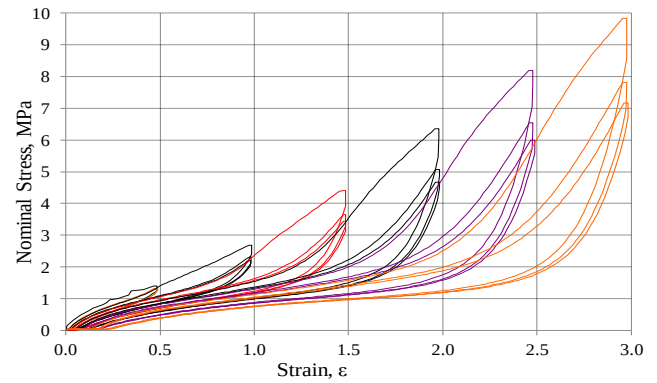
Fig. 11. Stress-strain in simple extension for A4 from zero strain.
