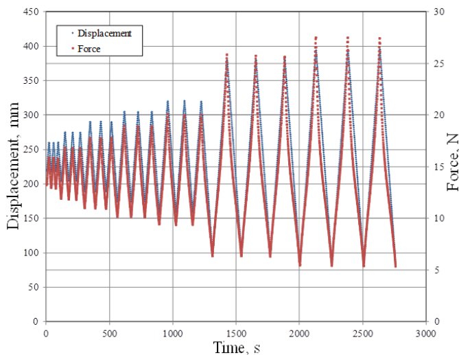
Fig. 3. Example of displacement-time plot of cyclic test for A6 compound.
