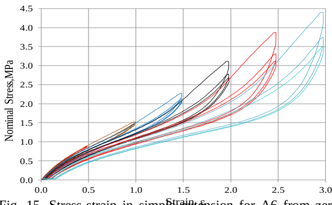
Fig. 15. Stress-strain in simple extension for A6 from zero strain.
