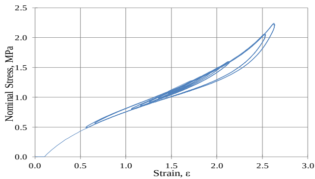
Fig. 7. Stress-strain in simple extension for A2 from zero strain.
