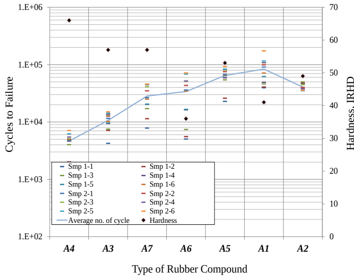
Fig. 20. Overall fatigue test results of all rubber compounds at 160 \pm 105\% strain. The relationship of fatigue test results and hardness was plotted for comparison.
