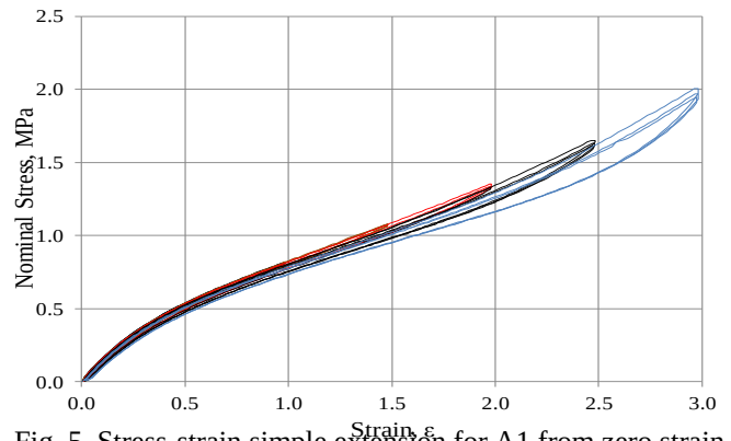
Fig. 5. Stress-strain simple extension for A1 from zero strain.
