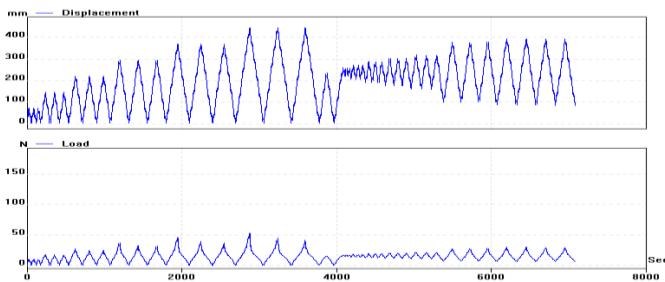
Fig. 3. Example of displacement-time plot of cyclic test for A6 compound.
