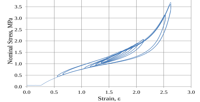
Fig. 12. Typical non-relaxing stress-strain of A4 at strain amplitude of 15%, 25%, 35%, 45%, 55%, 95% and 105%.
