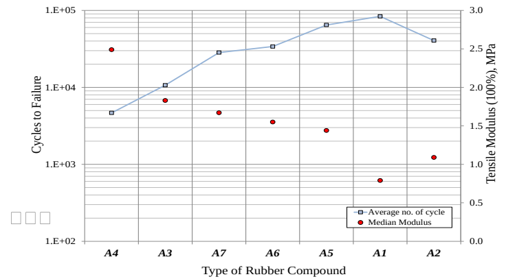
Fig. 23. Overall fatigue test results of all rubber compounds at 160 \pm 105\% strain. The relationship of fatigue test results and tensile modulus was plotted for comparison.
