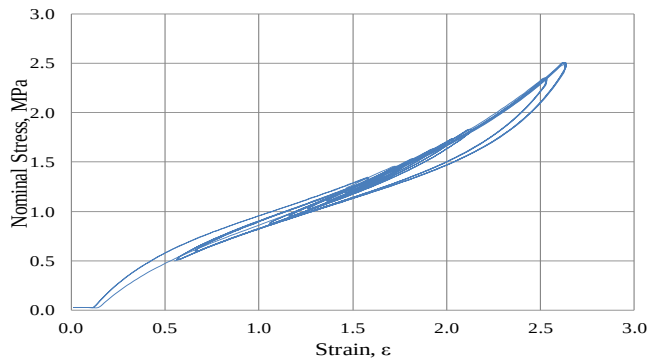
Fig. 16. Typical non-relaxing stress-strain of A6 at strain amplitude of 15%, 25%, 35%, 45%, 55%, 95% and 105%.
