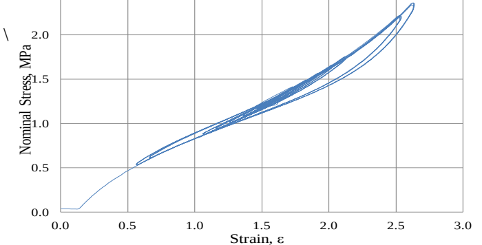
Fig. 13. Stress-strain in simple extension for A5 from zero strain.
