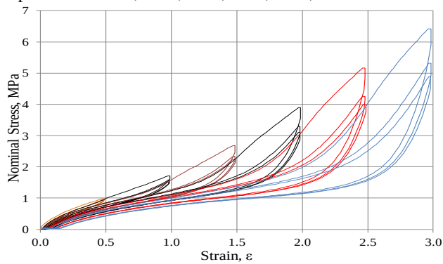
Fig. 8. Typical non-relaxing stress-strain of A2 at strain amplitude of 15%, 25%, 35%, 45%, 55%, 95% and 105%.
