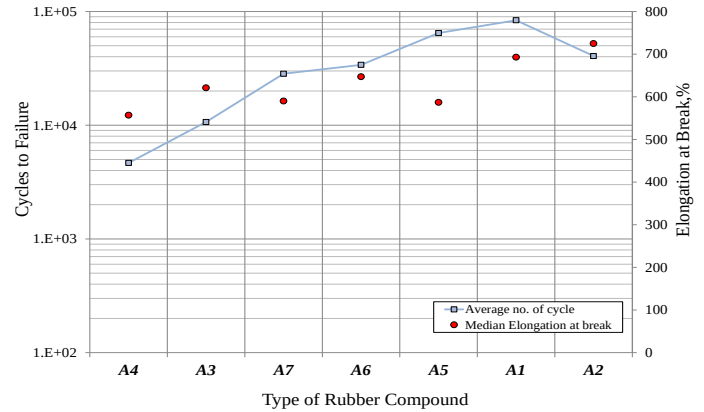
Fig. 22. Overall fatigue test results of all rubber compounds at 160 \pm 105\% strain. The relationship of fatigue test results and elongation at break was plotted for comparison.
