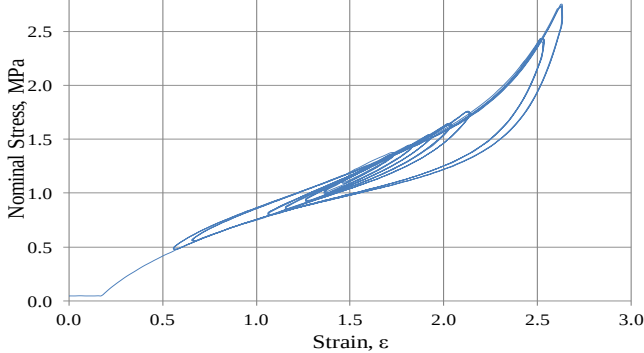
Fig. 9. Stress-strain in simple extension for A3 from zero strain.
