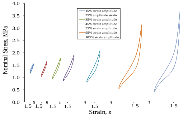
Fig. 19. Separation of stress-strain curves for each strain amplitude A4.
