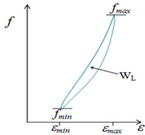
Fig. 1. Hysteresis loop showing non-linear behaviour typical of filled rubber at high strain [6].
