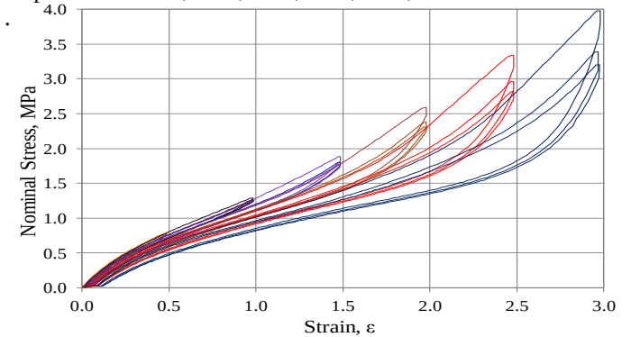
Fig. 13. Stress-strain in simple extension for A5 from zero strain.
