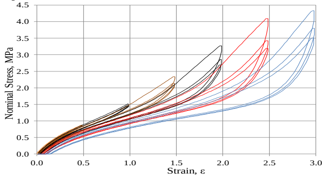
Fig. 17. Stress-strain in simple extension for A7 from zero strain.
