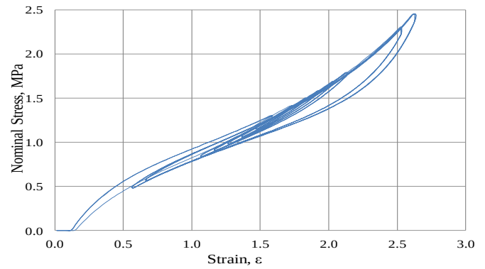
Fig. 18. Typical non-relaxing stress-strain of A7 at strain amplitude of 15%, 25%, 35%, 45%, 55%, 95% and 105%.
