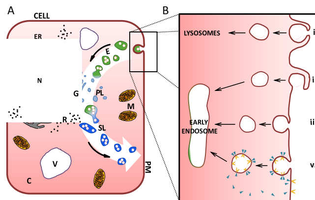
Figure 3: (A) A schematic of a cell highlights different compartment. The endocytotic pathway is indicated by the white arrow in the background. After internalisation of the cargo into membrane-bound vesicles inside the cell (light-green, (B) for more details), these vesicles fuse to early endosomes and mature to late endosomes, here shown as green vesicles. Primary lysosomes (abbr. PL, here with light blue colouration) emerge from the Golgi apparatus (G) and merge with endosomes (E, green colouration) to form secondary lysosomes (SL, darker blue colouration). Passing through maturation and degradation processes, they get eventually exocytosed by the cell. (B) Detailed schematic showing the main mechanisms of endocytosis featuring phagocytosis (i), macropinocytosis (ii), non-specific absorptive endocytosis (iii) and receptor-mediated endocytosis (vi) involving receptor (yellow shape) and coating molecules (e.g. clathrin- and caveolin, blue triangle). Abbr.: cytoplasm (C), early and late endosomes (E), endoplasmic reticulum (ER), Golgi apparatus (G), mitochondria (M), nucleus (N), primary lysosome (PL), plasma membrane (PM), ribosome (R), secondary lysosome (SL), vacuole (V). Figure is not to scale.
