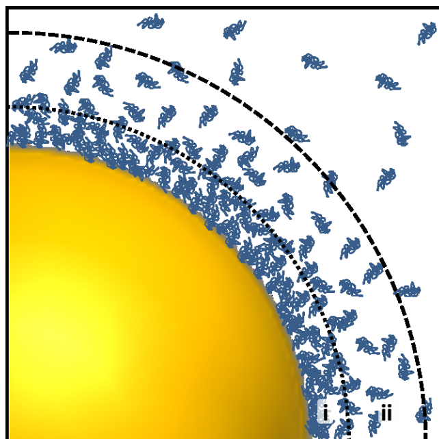
Figure 4: Illustration of the protein corona around a spherical gold nanoparticle in a protein-rich environment. Proteins, here shown as blue entangled chains, adhere to the particle's surface forming a 'hard' (i) and 'soft' (ii) layer. While the inner 'hard' layer consists of proteins strongly adsorbed to the particle's surface, the outer 'soft' layer is formed by weak protein-protein interactions.
