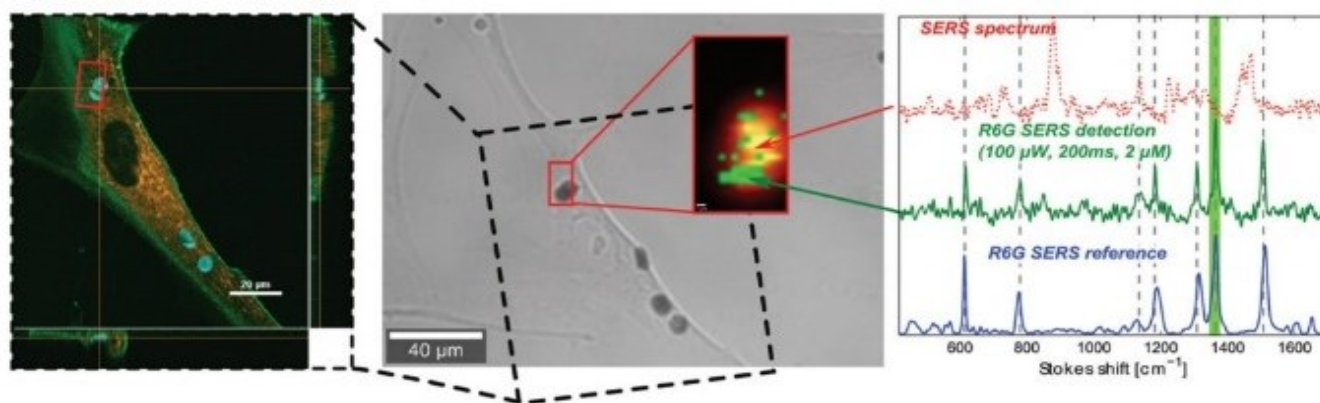
Figure 9: Reporter-free intracellular detection of Rhodamine-6G. (A) Confocal fluorescence scan of a single cell with several nanodome-patterned microchips show the intracellular localisation of the microchips, as well as the uptake and inhomogeneous distribution of R6G in the cell. (B) Transmission image of the same cell, where SERS spectra are mapped over the region marked with a red square. The inset shows the integrated number of counts in the 400–1700 \text{cm}^{-1} region (graded red-yellow), on top of which the presence of the 1365 \text{cm}^{-1} R6G-peak is highlighted in green, which corresponds to the green shaded area in (C). (C) SERS spectra on different positions of the microchip show the intracellular SERS detection of R6G (middle, green) and the R6G reference SERS spectrum (bottom, blue), while other positions show the presence of peaks related to other molecules adsorbed on the microchip (dotted red, top). Spectra are normalized and offset for clarity. Reprinted with permission from P. C. Wuytens, A. Z. Subramanian, W. H. De Vos, A. G. Skirtach and R. Baets, The Analyst , 2015- Published by The Royal Society of Chemistry.
