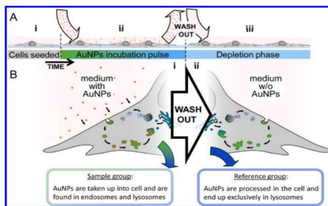
Figure 7: Schematic of experimental design. (A) Full experimental procedure involves AuNPs (red spheres) being added to the cell culture environment after (A.i) cells have sufficiently attached to the culture dish. (A.ii) Following uptake of the particles into the cell via endocytosis during the incubation pulse, extracellular particles were washed out. (A.iii) Fresh culture medium without AuNPs was added and the cells were left until incorporated particles were processed into lysosomes (depletion phase). (B.i) During the incubation phase, cells constantly internalize AuNPs, which accumulate inside endosomes (green vesicles) and lysosomes (blue vesicles). Their acquired SERS map data serves as the sample group for analysis. (B.ii) Following the wash-out, vesicular AuNPs are processed along the endolysosomal pathway and are eventually found exclusively in lysosomes. SERS maps of cells with only lysosomal AuNPs serve as the reference group for the data analysis. Reprinted with permission from A. Huefner, W.-L. Kuan, K. H. Müller, J. N. Skepper, R. A. Barker and S. Mahajan, ACS Nano , 2015. Copyright 2015 ACS Nano.
