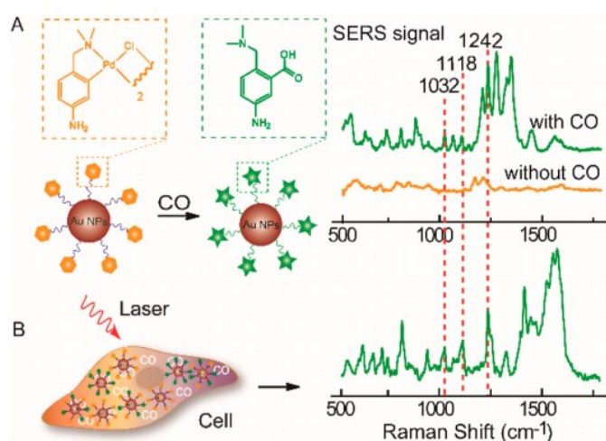
Figure 5: (A) SERS response and sensing mechanism of palladacycle carbonylation on AuNP/PC nanosensors for CO. (B) SERS detection of CO in living cells using AuNP/PC nanosensors. Reprinted with permission from Y. Cao, D.-W. Li, L.-J. Zhao, X.-Y. Liu, X.-M. Cao and Y.-T. Long, Anal. Chem. , 2015, 87 , 9696–9701. Copyright (2015) Anal. Chem
