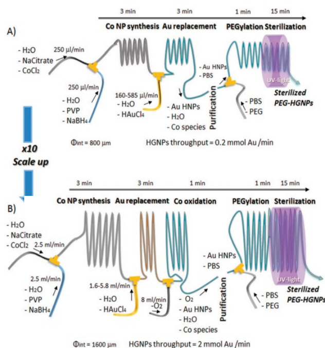
Figure 2 Experimental set up for the production of HGPNs produced from galvanic replacement of sacrificial Co templates, including stages PEG functionalisation and sterilisation on a singular platform, scaled up for high throughput. Reprinted with permission from L. Gomez, V. Sebastian, S. Irujo, A. Ibarra, M. Arruebo and J. Santamaria, Lab Chip , 2014, 14 , 325–332. Copyright (2014) Lab Chip.
