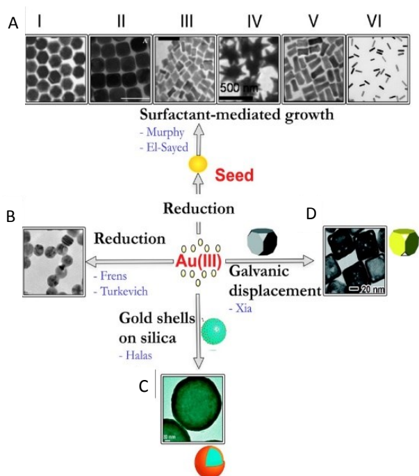
Figure 1 Representative synthetic approaches to prepare AuNPs with controllable size and shape. (A) Surfactant-mediated solution-based growth method to prepare AuNPs with hexagonal (A, I), cubic (A, II), rectangular (A, III), star (A, IV), dog bone (A, V), and rod (A, VI) shapes. (B) Citrate-mediated growth method to prepare Au nanospheres via direct reduction of Au ions. (C) Sequential growth method to prepare Au nanoshell on silica. (D) Galvanic replacement reaction on the surface of Ag nanocubes to prepare porous/hollow Au nanocages. Reprinted with permission from Alkilany et al. Acc. Soc. Res. 2013, 46, 650-661. Copyright (2013) American Chemical Society. Images in A and D are reprinted with permission from references 25 and 35 respectively; Copyright (2004, 2011, respectively) American Chemical Society. Images in C is reprinted with permission from Wang et al. Acc. Chem. Res. 2007, 40, 5362; Copyright (2007) American Chemical Society.
