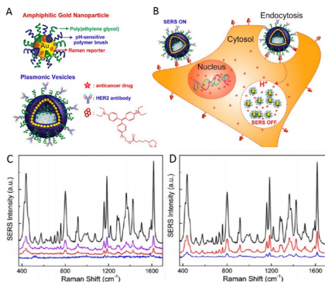
Figure 6 (A) Schematic illustration of the amphiphilic gold nanoparticle coated with Raman reporter BGLA and mixed polymer brushes of hydrophilic PEG and pH-sensitive hydrophobic PMMAVP grafts and the drug-loaded plasmonic vesicle tagged with HER2 antibody for cancer cell targeting. (B) The cellular binding, uptake, and intraorganelle disruption of the SERS-encoded pH-sensitive plasmonic vesicles. (C) Representative SERS spectra of SKBR-3 cells treated with HER2-targeted vesicles (black line) and untargeted vesicle (purple line), MCF-7 cells treated with targeted vesicles (red line), and SKBR-3 control cells (blue line). (D) Representative SERS spectra of SKBR-3 cells labeled with targeted vesicles after 30 min incubation (black line) and the postincubation spectra of the cells at 60 min (red line) and 90 min (blue line). Reprinted with permission from J. Song, J. Zhou and H. Duan, J. Am. Chem. Soc. , 2012, 134 , 13458–13469. Copyright 2012 J. Am. Chem. Soc.
