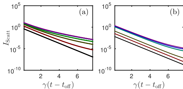
FIG. 6. The simulated scattered power collected by the lens as a function of time after a 125 ns square excitation pulse is turned off for (a) a homogeneously broadened sample, and (b) an inhomogeneously broadened sample of ^{87}\text{Rb} atoms with the Doppler broadening of 100\gamma . Here the atoms are trapped in a thermal equilibrium during and after the pulse. We show the intensity scattered into the detection apparatus (the curves from bottom to top) for the atom numbers N = 1 (black), N = 5 (red), N = 20 (brown), N = 50 (green), N = 200 (cyan), N = 325 (blue), and N = 450 (purple). The light is on single-atom resonance. The varying rates of decay in the homogeneously broadened sample indicate the participation of both superradiant and subradiant collective modes, while the constant decay rates of the inhomogeneously broadened samples at the lowest atom numbers indicate that the atoms are radiating independently.
