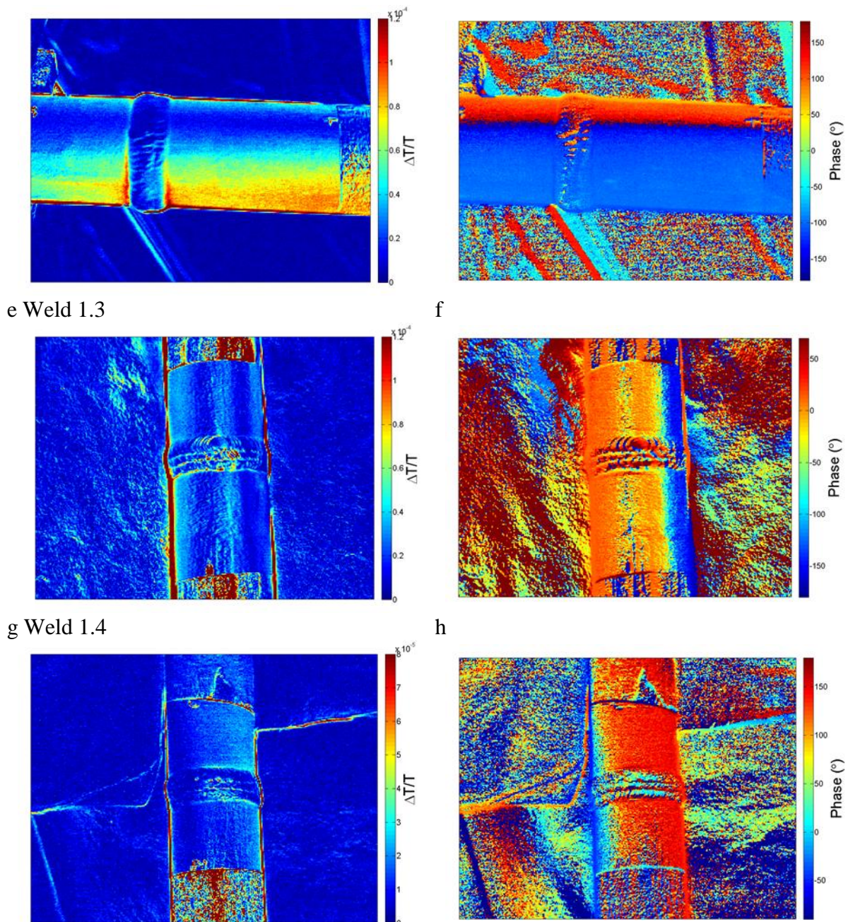
Figure 16: TSA \Delta T/T and phase results for welds 1.1 – 1.4 on pipe 1.
