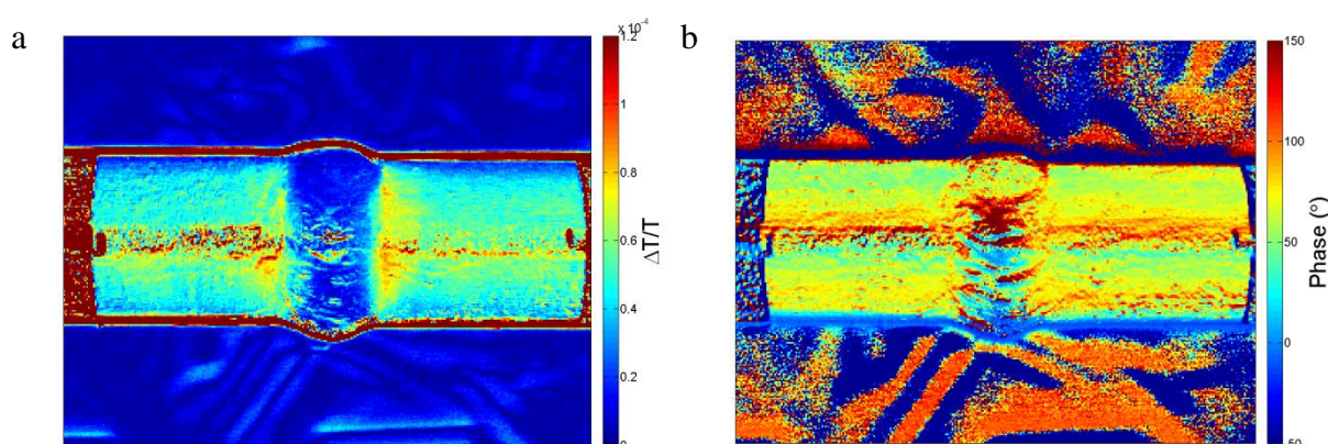
Figure 17: TSA a) \Delta T/T and b) phase results for weld 2.1 on pipe 2.
