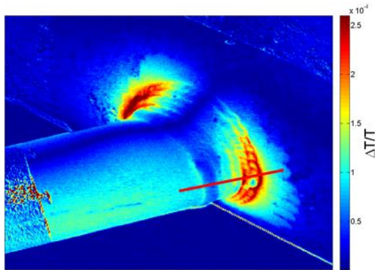
c Weld 1.2
