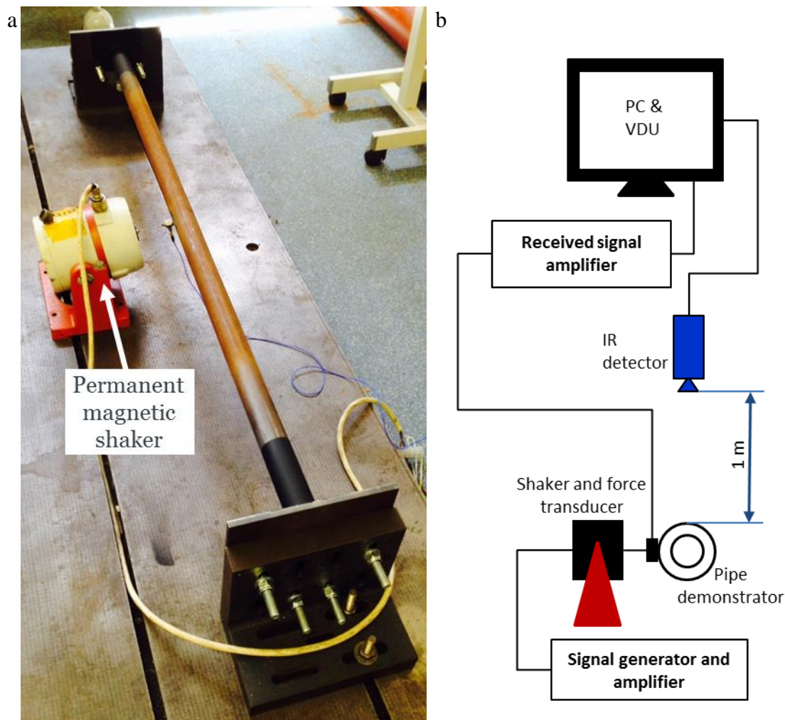
Figure 7: Demonstrator I a) photograph of shaker positioning and b) schematic of full experimental set up.
