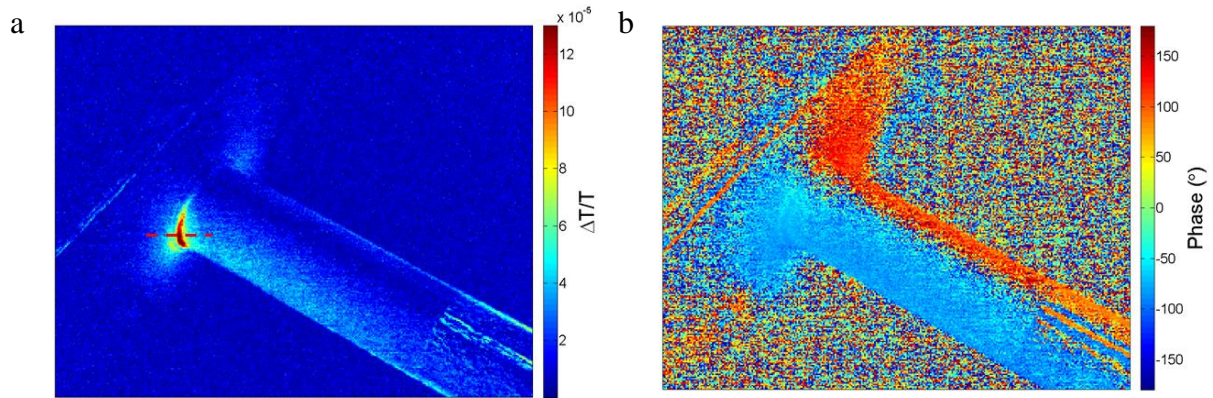
Figure 9: a) TSA \Delta T/T and b) phase results for demonstrator I.
