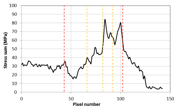
Figure 18 Weld 1.1 stress sum data calculated along the profile line in Figure 16a with weldment edges (red dashed line) and position of each weld pass (orange dashed line) marked.
