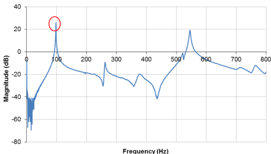
Figure 6: Transfer function used to identify the first mode excitation frequency for the permanent magnetic shaker.
