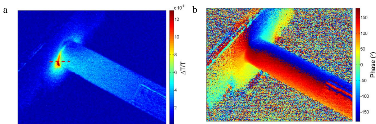
Figure 11: a) TSA \Delta T/T and b) phase results for demonstrator II.
