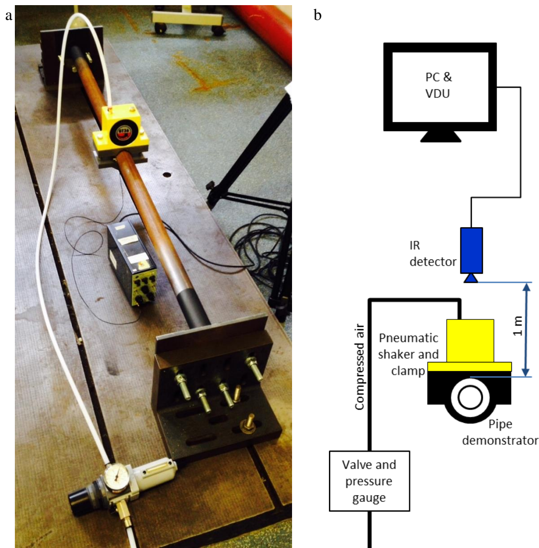
Figure 8: Demonstrator II a) photograph of pneumatic shaker positioning and b) schematic of full experimental set up.
