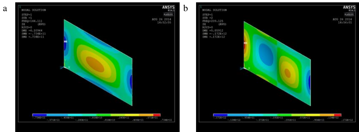
Figure 2: FEA modal analysis results determining the frequencies of a) mode 1 and b) mode 2.
