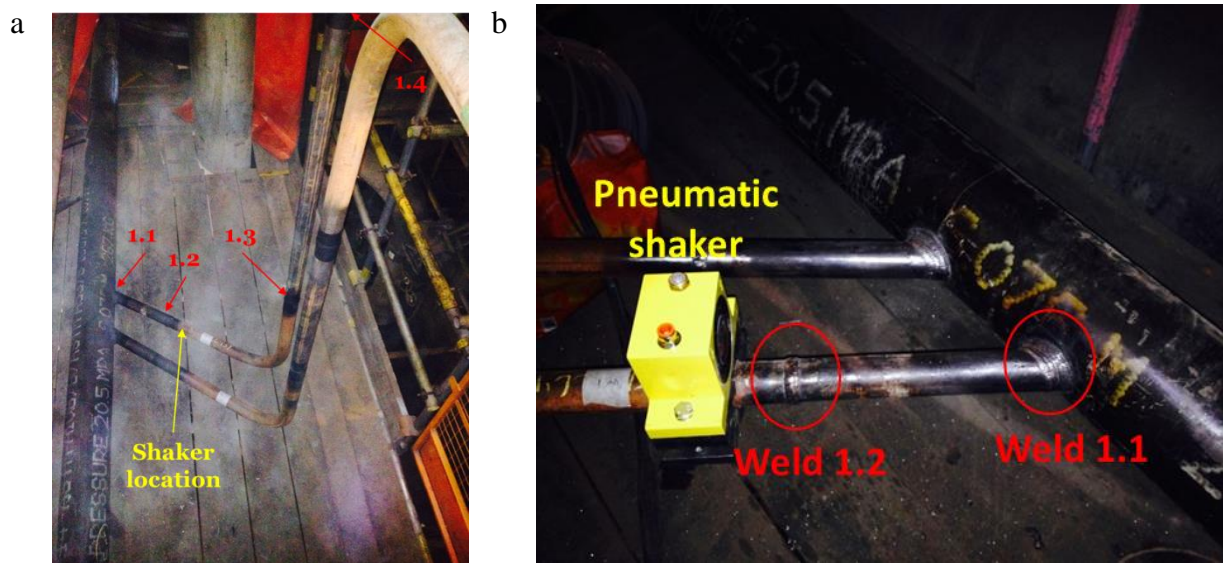
Figure 14: a) weld and shaker locations highlighted on pipe 1, b) shaker position on pipe 1 with welds 1.1 and 1.2 highlighted.
