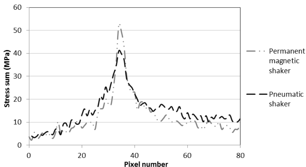
Figure 12: Stress sum profiles taken across the weld for demonstrators I and II.
