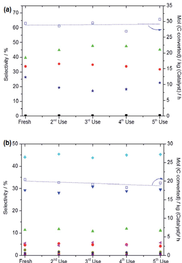
Fig. 8 Catalytic performance of 1.1 wt% Fe/ZSM-5_#4 employed in the oxidation of (a) methane and (b) ethane using H_2O_2 as oxidant over five (5) reuse cycles. Test conditions for (a) 27 mg catalyst; reaction volume: 10 ml; [H_2O_2] : 0.5 M; reaction temperature: 50 °C; time: 0.25 h; stirring rate: 1500 rpm, P(CH_4) : 30 bar. Test conditions for (b) 54 mg catalyst; reaction volume: 20 ml; [H_2O_2] : 1 M; reaction temperature: 30 °C, time: 0.5 h, stirring rate: 1500 rpm; P(C_2H_6) : 5 bar.
