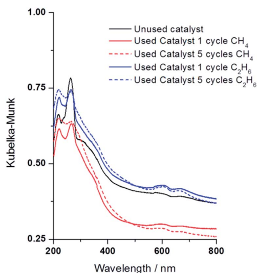
Fig. 9 DR UV-vis spectra of 1.1 wt% Fe/ZSM-5_#4 employed in the oxidation of methane and ethane measured after one (1) and five (5) reaction cycles using \text{H}_2\text{O}_2 as oxidant. Test conditions as in Fig. 8, catalysts analysed at room temperature after air drying overnight.
