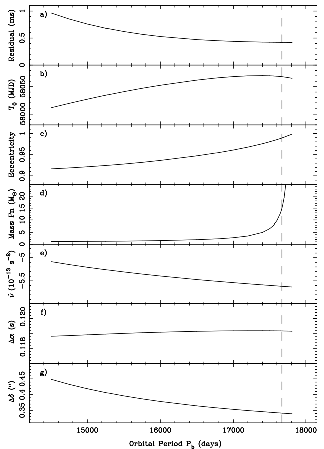
Figure 2. Results of fits to TOAs of a number of binary models having different fixed values of orbital period P_b : a) Rms timing residual \sigma_t , b) epoch of periastron T_0 , c) orbital eccentricity \epsilon , d) mass function f_m , e) pulsar rotational frequency derivative \dot{\nu} , f) deviation of right ascension of pulsar \Delta\alpha from 20^{\text{h}}32^{\text{m}}13^{\text{s}} , g) deviation of declination \Delta\delta from 41^\circ27'24'' . Solutions to the right of the vertical dashed line (at P_b = 17670 d) are disallowed by the pulsar and Be star masses ( f_m \leq 15 M_\odot ; see text). Parameters for P_b = 16000 (Model 1), 17000 (Model 2), and 17670 d (Model 3) are given in Table 1.
