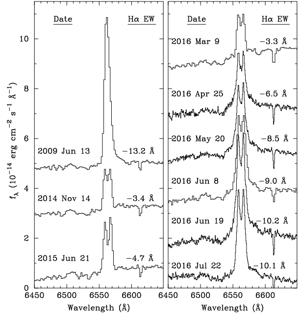
Figure 7. H \alpha region of spectra of MT91 213 (see Table 5). Spectra have been shifted vertically for clarity. 2009 spectrum is the same as appears in Camilo et al. (2009). Absolute flux densities for MDM spectra are not reliable due to the narrow ( 1'' ) slit width used.
