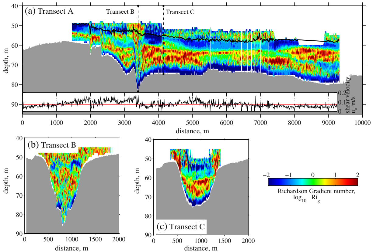
Fig. 6. (a)–(c) Turbulent mixing in Transects A–C respectively, as parameterized by the Richardson gradient number, Ri_g . Inset shows shear velocity, u_* , calculated at 1 m above the bed with mean shear velocity denoted by a solid red line. In (a) dashed black lines denote the location of the cross-sectional Transects B and C. In (a)–(c) solid black curves denote the top of the flow, as defined by the contour of zero downstream flow velocity. (For interpretation of the references to colour in this figure legend, the reader is referred to the web version of this article.)
