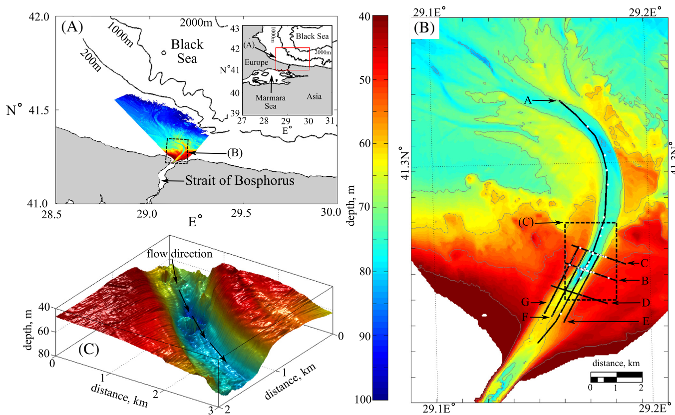
Fig. 1. (a) The location of the field site, in the southwest Black Sea (bathymetry data from GEBCO, 2014). (b) A bathymetric map of the channel system showing depth below sea-level, ADCP Transects A–G, denoted by solid black lines, and locations of CTD profiles, denoted by white circles. (c) Three-dimensional visualization of the channel system, at the location of the largest hydraulic jump located at the intersection of Transects A and B.
