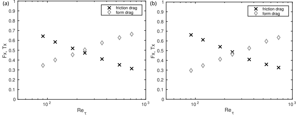
FIGURE 10. Frictional and form drag for the rough surfaces: (a) graphite, (b) gritblasted surface.
