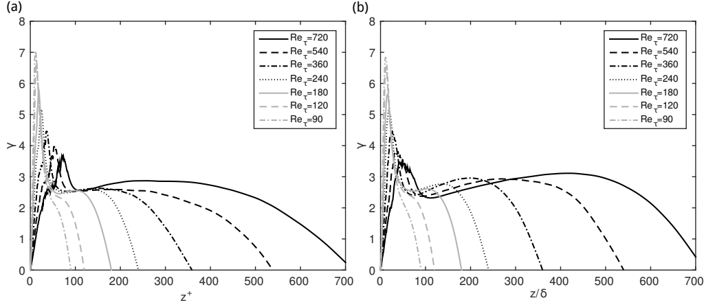
FIGURE 6. Diagnostic quantity for a log-law: (a) graphite case, (b) gritblasted case.
