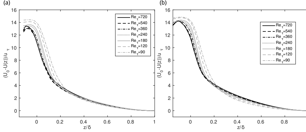
FIGURE 5. Mean velocity defect profiles: (a) graphite case, (b) gritblasted case.
