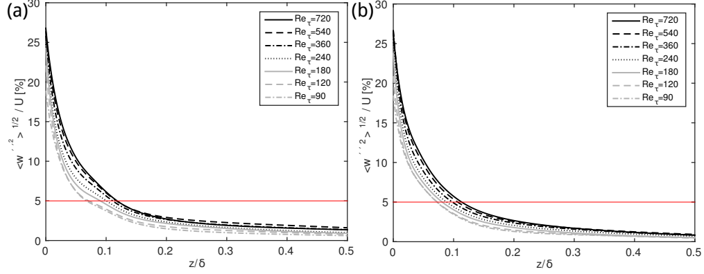
FIGURE 12. Standard deviation of time-averaged wall-normal velocity normalised by streamwise mean velocity (percentage values). (a) graphite surface, (b) gritblasted surface. The horizontal red line shows the 5% level.
