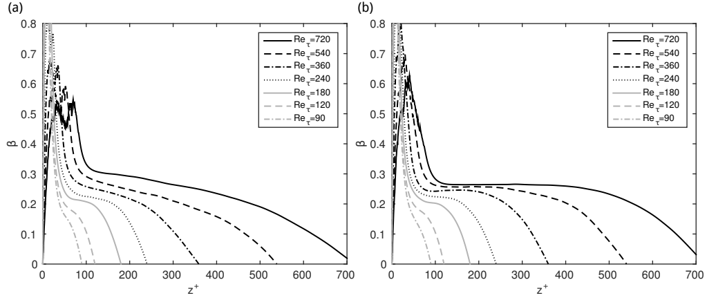
FIGURE 7. Diagnostic quantity for a power-law: (a) graphite case, (b) gritblasted case.
