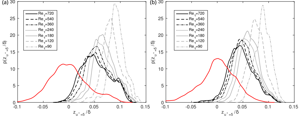
FIGURE 14. Location of the upper end of the blanketing layer: (a) graphite surface, (b) gritblasted surface. The red curves show the pdfs for the surface height distributions.
