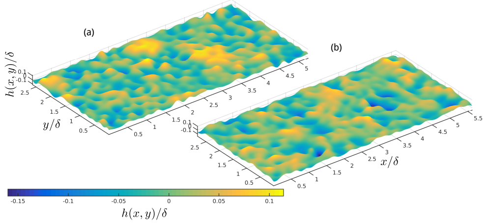
FIGURE 1. Topographies of the rough surfaces: (a) graphite surface, (b) gritblasted surface.
