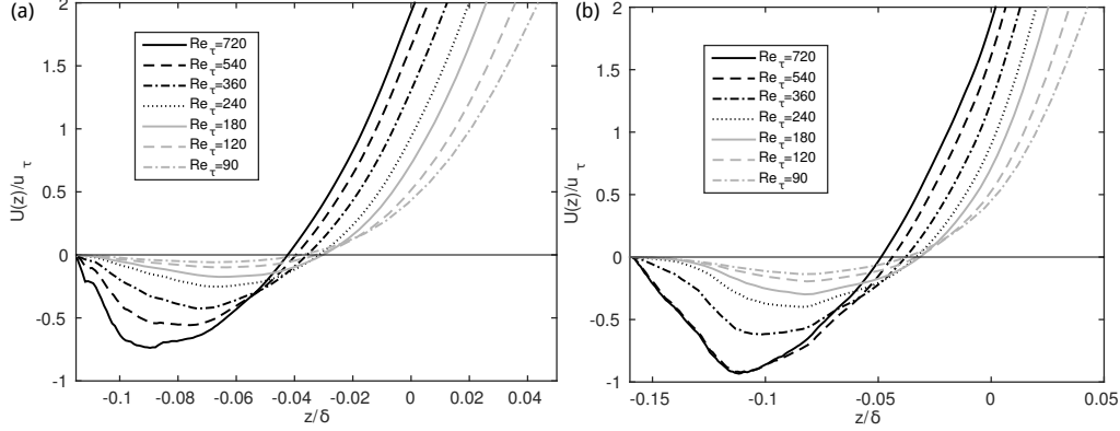
FIGURE 9. Mean velocity profiles in the near-wall region: (a) graphite case, (b) gritblasted case.
