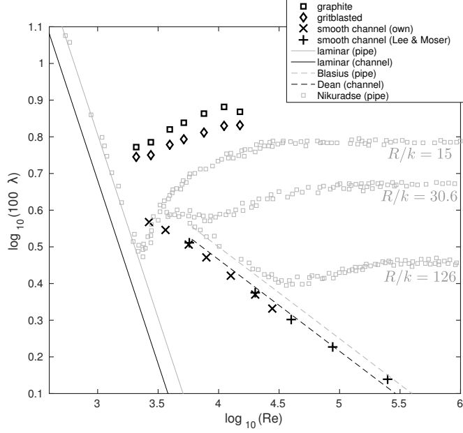
FIGURE 11. Variation of friction factor with Reynolds number, where \lambda is the friction factor (dimensionless pressure drop per unit length of channel/pipe) and Re is the bulk Reynolds number. For comparison, Nikuradse's data for different sand grain roughness heights relative to the pipe radius R and data from DNS of smooth-wall turbulent channel flow (including data from Lee & Moser (2015)). Also shown are the analytic relationships for the smooth wall laminar pipe and channel flow cases. The Blasius and Dean's relationships are shown for the fully developed smooth-wall turbulent pipe and channel flow cases.
