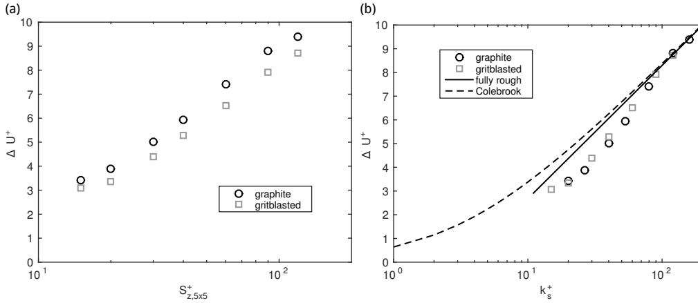
FIGURE 3. (a) Roughness function plotted vs mean-peak-to valley height; (b) roughness function vs estimated equivalent sand grain roughness, the fully rough asymptote and the Colebrook formula are shown for comparison.
