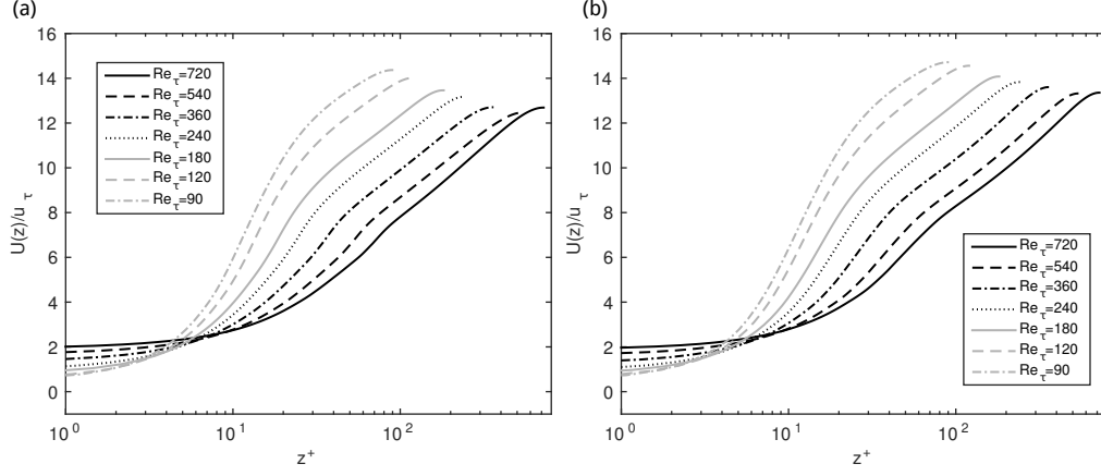
FIGURE 4. Semi-logarithmic profiles of mean streamwise velocity at different Reynolds numbers: (a) graphite surface, (b) gritblasted surface
