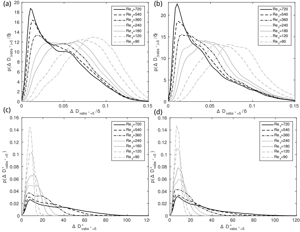
FIGURE 15. Pdf of thickness of blanketing layer. (a) and (c) graphite surface, (b) and (d) grit-blasted surface. Parts (a) and (b) show the thickness in outer units; parts (c) and (d) show the thickness in inner units.
