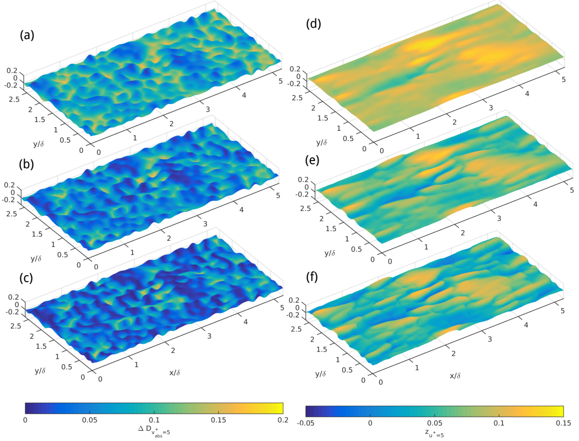
FIGURE 16. Graphite surface. (a)-(c) Rough surfaces coloured with thickness of blanketing layer. (a) Re_\tau = 90 , (b) Re_\tau = 240 , (c) Re_\tau = 720 . (d)-(f) Location of upper end of blanketing layer. (d) Re_\tau = 90 , (e) Re_\tau = 240 , (f) Re_\tau = 720 .
