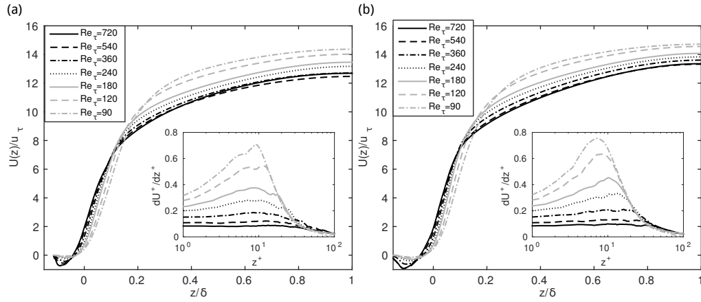
FIGURE 8. Mean velocity profiles with linear x-axis: (a) graphite case, (b) gritblasted case. The inset plots show the derivative of the mean velocity profile near the mean wall plane.
