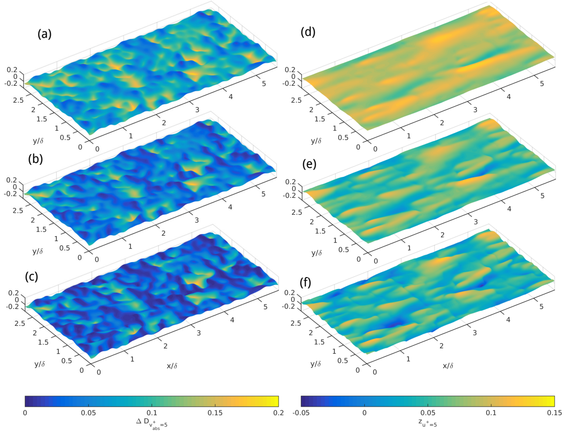
FIGURE 17. Gritblasted surface. (a)-(c) Rough surfaces coloured with thickness of blanketing layer. (a) Re_\tau = 90 , (b) Re_\tau = 240 , (c) Re_\tau = 720 . (d)-(f) Location of upper end of blanketing layer. (d) Re_\tau = 90 , (e) Re_\tau = 240 , (f) Re_\tau = 720 .
