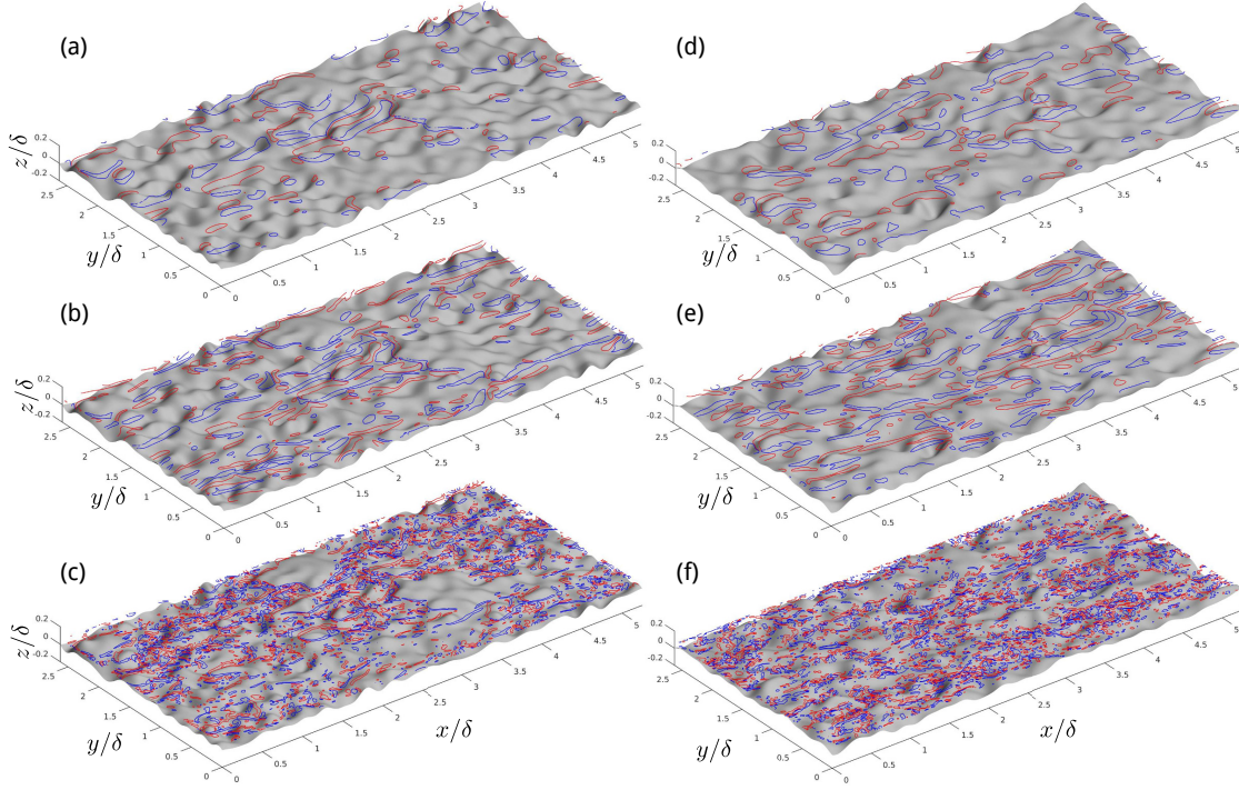
FIGURE 20. Contours of the wall-normal component of the instantaneous vorticity \omega_z (red: +1\sigma_{\omega_z} , blue: -1\sigma_{\omega_z} ) shown in the plane z/\delta = 0.05 . Left column: graphite surface; right column: gritblasted surface. (a) and (d): Re_\tau = 90 ; (b) and (e): Re_\tau = 240 ; (c) and (f): Re_\tau = 720
