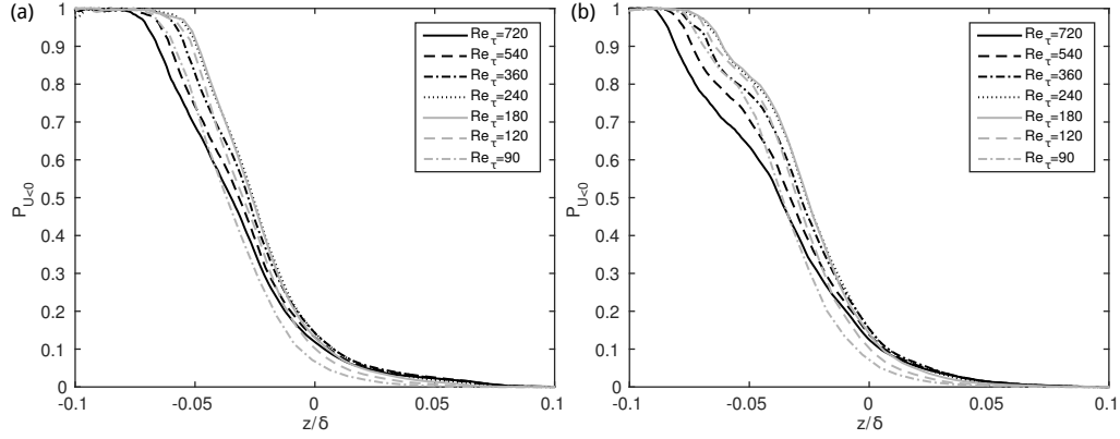
FIGURE 13. Probability of negative \bar{u} versus wall-normal coordinate z for different Reynolds numbers: (a) graphite case, (b) gritblasted case
