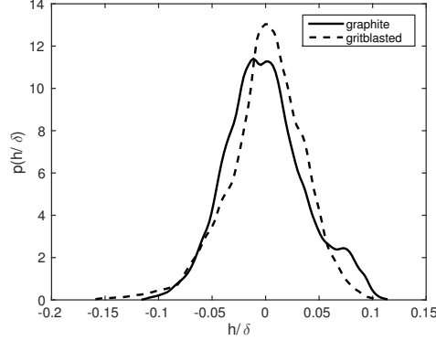
FIGURE 2. Height distribution of the graphite and the gritblasted surface.
